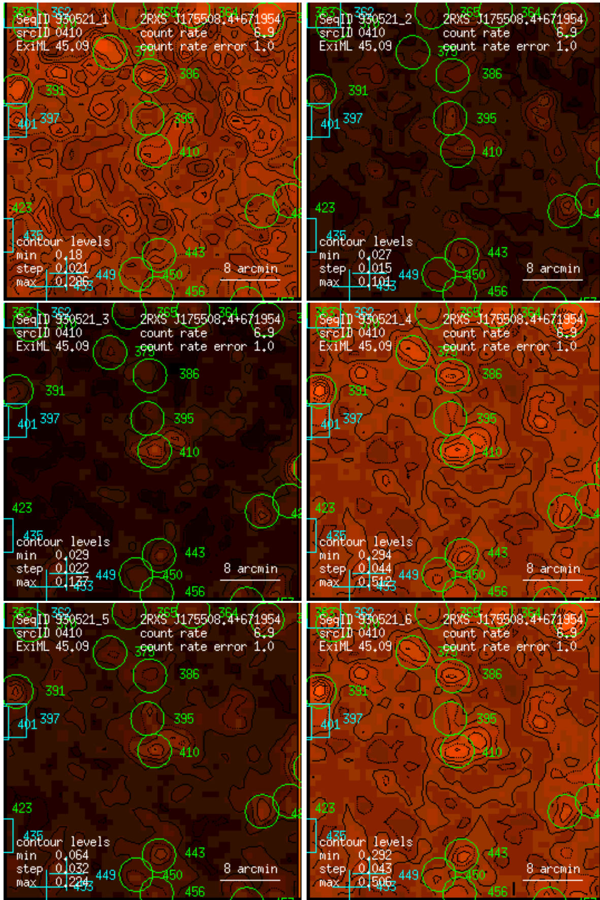
Figure 410: RASS 930521: detection 0410: band rate images, Gaussian filter: (1) PSPC channels 11 – 41, (2) 52 – 90, (3) 91 – 201, (4) 11 – 235, (5) 52 – 201, (6) 11 – 201. Broad band rates in counts/ks. Band rate contour levels in counts/ks/arcmin 2 .
