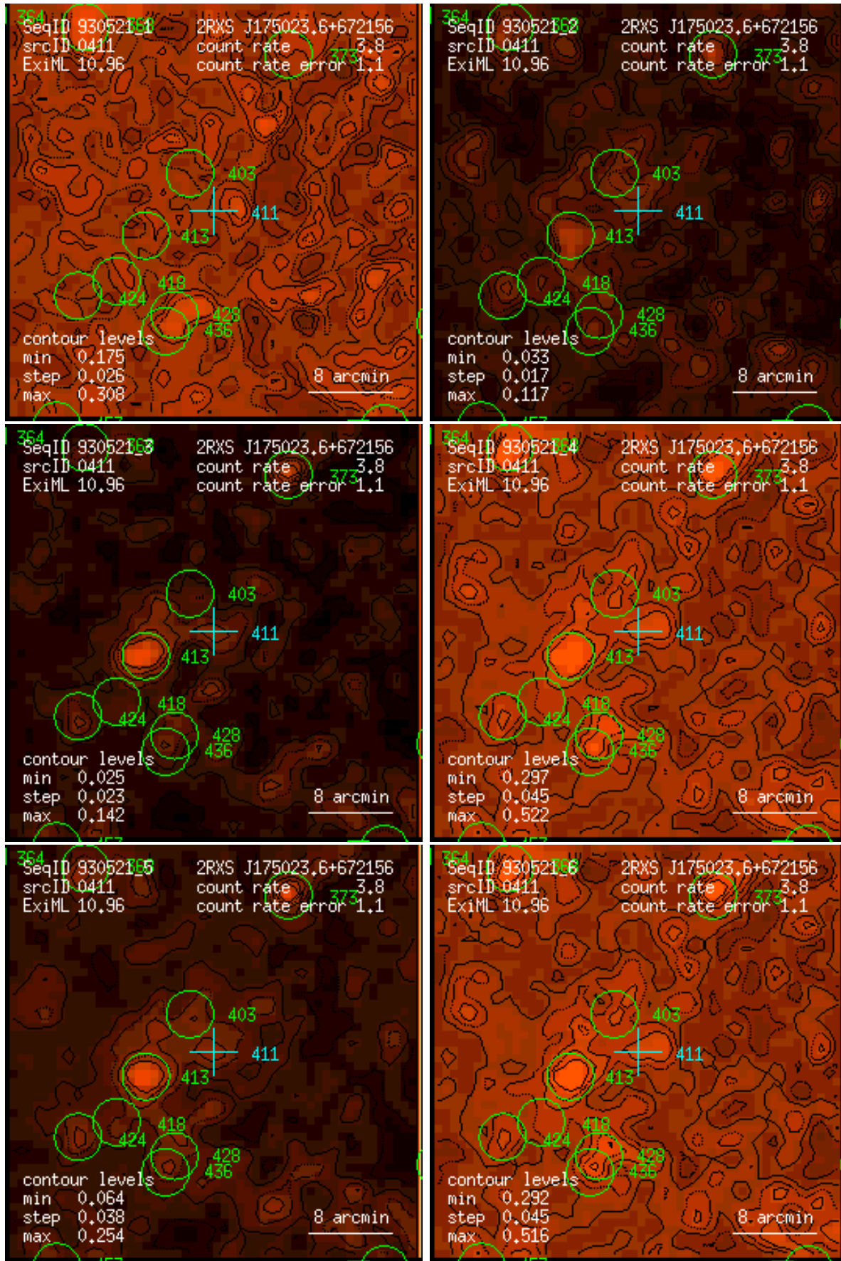
Figure 411: RASS 930521: detection 0411: band rate images, Gaussian filter: (1) PSPC channels 11 – 41, (2) 52 – 90, (3) 91 – 201, (4) 11 – 235, (5) 52 – 201, (6) 11 – 201. Broad band rates in counts/ks. Band rate contour levels in counts/ks/arcmin 2 .
