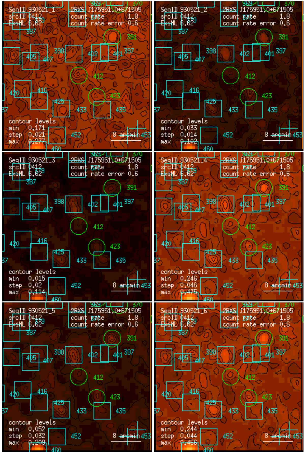
Figure 412: RASS 930521: detection 0412: band rate images, Gaussian filter: (1) PSPC channels 11 – 41, (2) 52 – 90, (3) 91 – 201, (4) 11 – 235, (5) 52 – 201, (6) 11 – 201. Broad band rates in counts/ks. Band rate contour levels in counts/ks/arcmin 2 .
