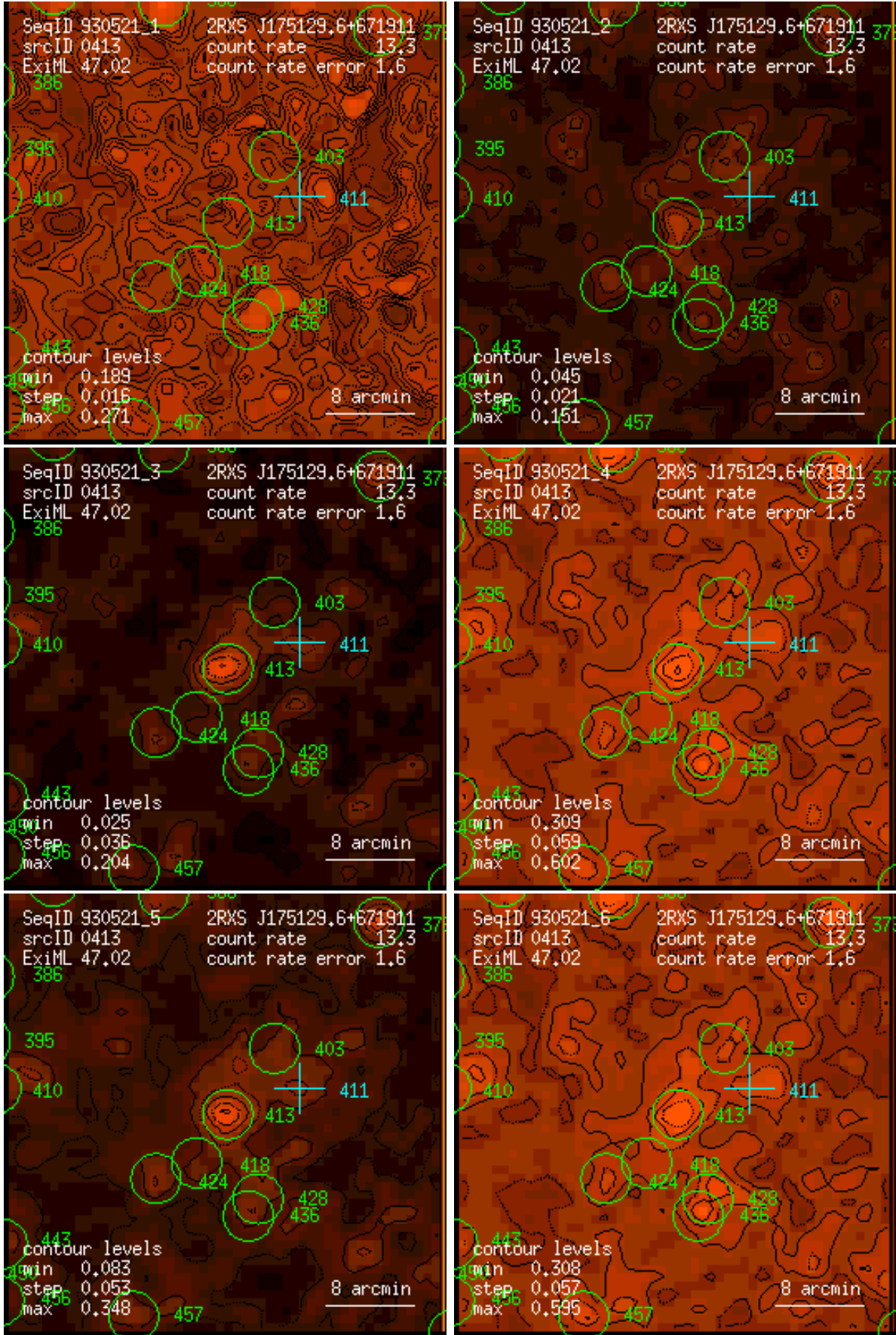
Figure 413: RASS 930521: detection 0413: band rate images, Gaussian filter: (1) PSPC channels 11 – 41, (2) 52 – 90, (3) 91 – 201, (4) 11 – 235, (5) 52 – 201, (6) 11 – 201. Broad band rates in counts/ks. Band rate contour levels in counts/ks/arcmin 2 .
