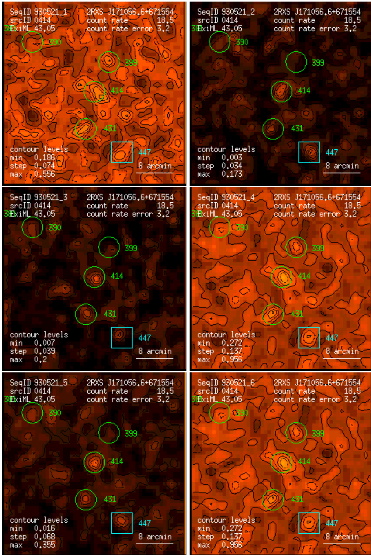
Figure 414: RASS 930521: detection 0414: band rate images, Gaussian filter: (1) PSPC channels 11 – 41, (2) 52 – 90, (3) 91 – 201, (4) 11 – 235, (5) 52 – 201, (6) 11 – 201. Broad band rates in counts/ks. Band rate contour levels in counts/ks/arcmin 2 .
