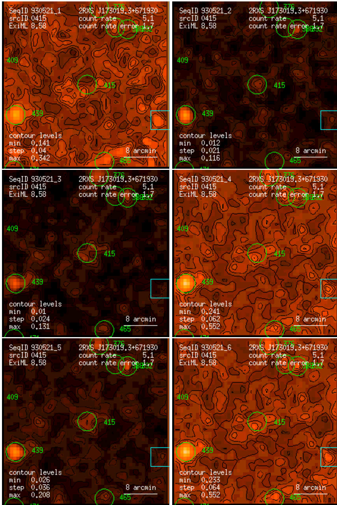
Figure 415: RASS 930521: detection 0415: band rate images, Gaussian filter: (1) PSPC channels 11 – 41, (2) 52 – 90, (3) 91 – 201, (4) 11 – 235, (5) 52 – 201, (6) 11 – 201. Broad band rates in counts/ks. Band rate contour levels in counts/ks/arcmin 2 .
