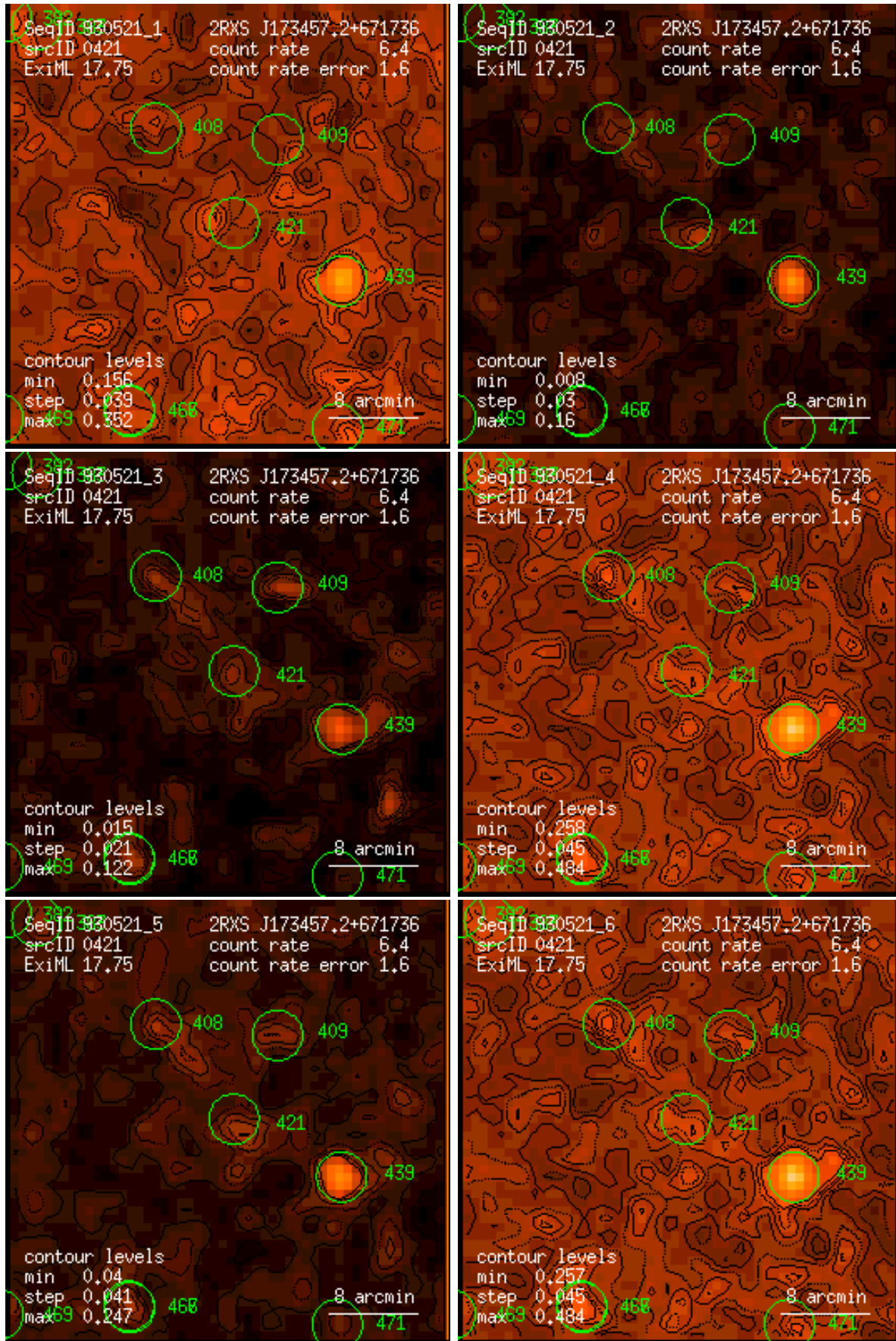
Figure 421: RASS 930521: detection 0421: band rate images, Gaussian filter: (1) PSPC channels 11 – 41, (2) 52 – 90, (3) 91 – 201, (4) 11 – 235, (5) 52 – 201, (6) 11 – 201. Broad band rates in counts/ks. Band rate contour levels in counts/ks/arcmin 2 .
