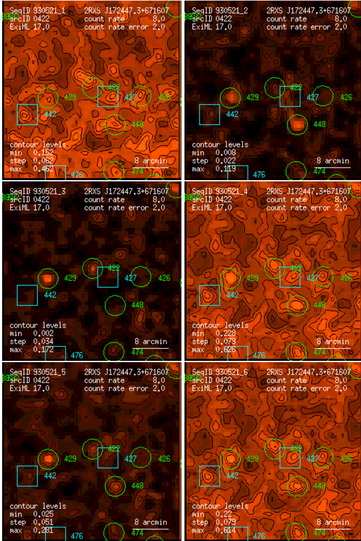
Figure 422: RASS 930521: detection 0422: band rate images, Gaussian filter: (1) PSPC channels 11 – 41, (2) 52 – 90, (3) 91 – 201, (4) 11 – 235, (5) 52 – 201, (6) 11 – 201. Broad band rates in counts/ks. Band rate contour levels in counts/ks/arcmin 2 .
