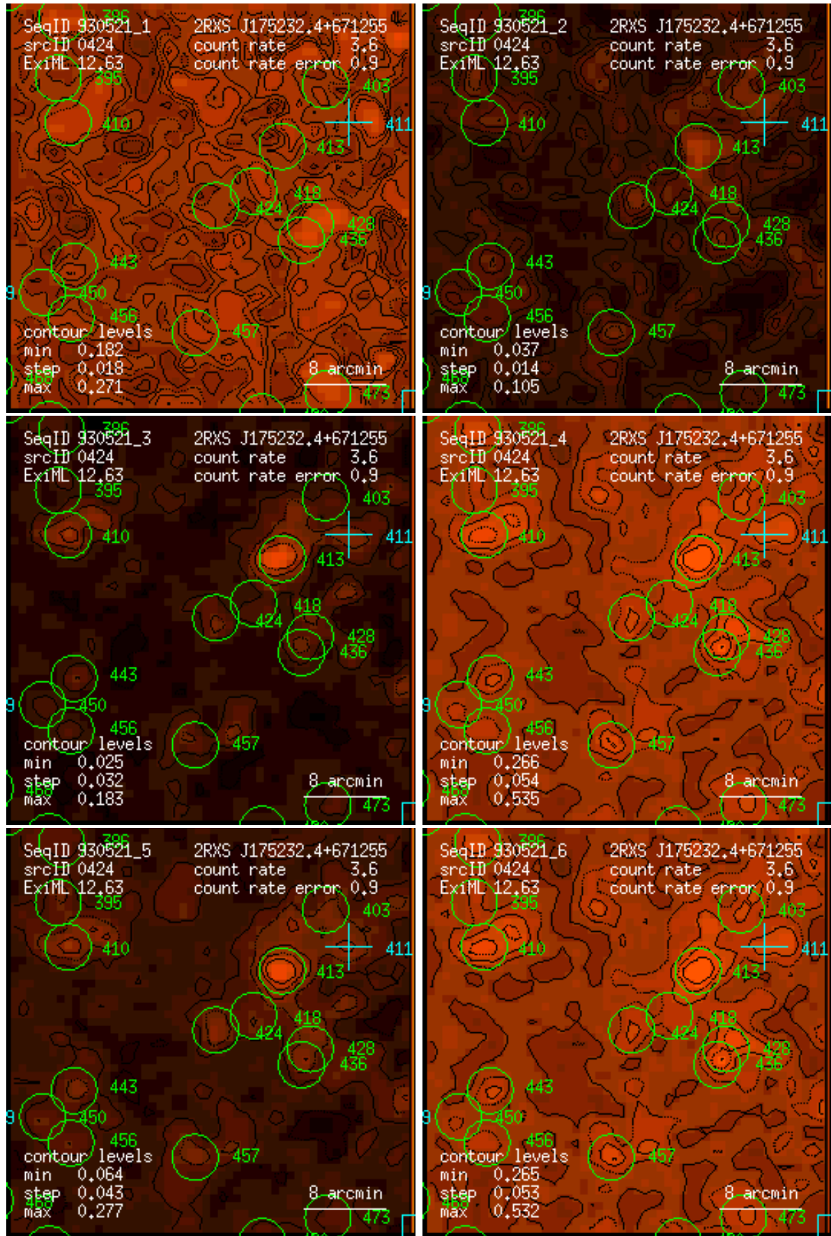
Figure 424: RASS 930521: detection 0424: band rate images, Gaussian filter: (1) PSPC channels 11 – 41, (2) 52 – 90, (3) 91 – 201, (4) 11 – 235, (5) 52 – 201, (6) 11 – 201. Broad band rates in counts/ks. Band rate contour levels in counts/ks/arcmin 2 .
