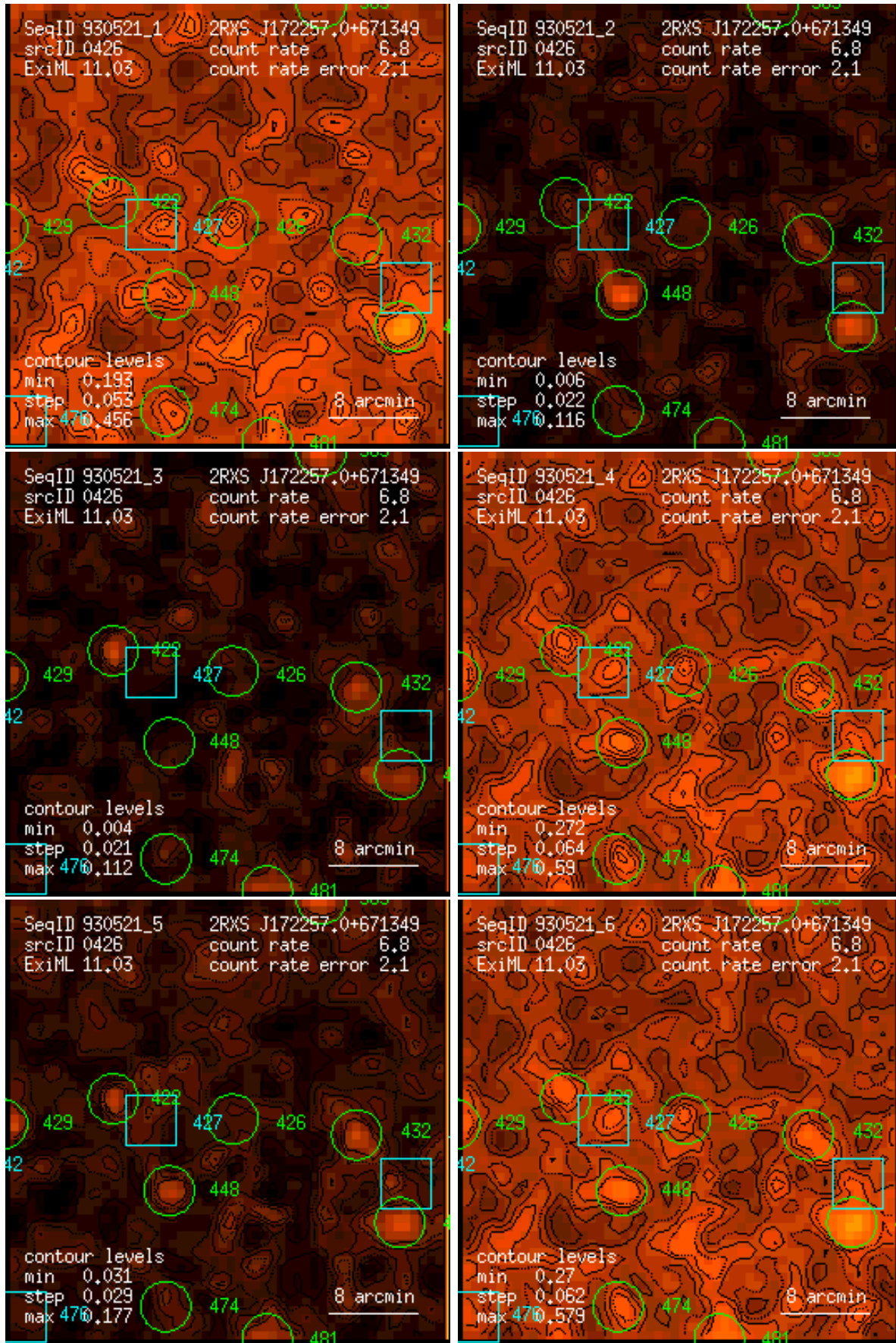
Figure 426: RASS 930521: detection 0426: band rate images, Gaussian filter: (1) PSPC channels 11 – 41, (2) 52 – 90, (3) 91 – 201, (4) 11 – 235, (5) 52 – 201, (6) 11 – 201. Broad band rates in counts/ks. Band rate contour levels in counts/ks/arcmin 2 .
