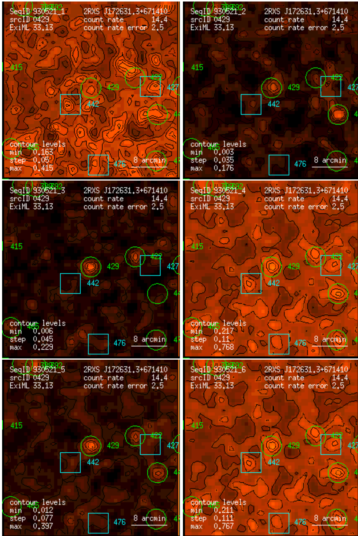
Figure 429: RASS 930521: detection 0429: band rate images, Gaussian filter: (1) PSPC channels 11 – 41, (2) 52 – 90, (3) 91 – 201, (4) 11 – 235, (5) 52 – 201, (6) 11 – 201. Broad band rates in counts/ks. Band rate contour levels in counts/ks/arcmin 2 .
