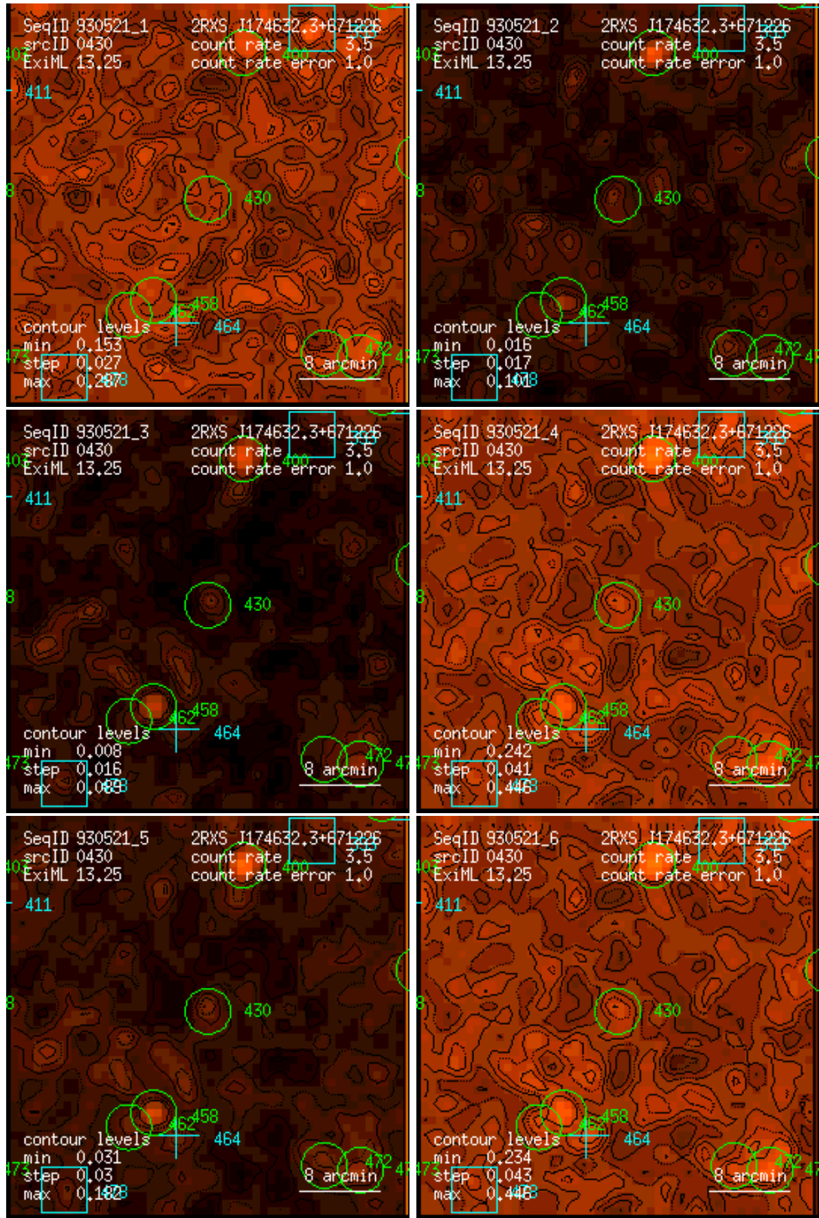
Figure 430: RASS 930521: detection 0430: band rate images, Gaussian filter: (1) PSPC channels 11 – 41, (2) 52 – 90, (3) 91 – 201, (4) 11 – 235, (5) 52 – 201, (6) 11 – 201. Broad band rates in counts/ks. Band rate contour levels in counts/ks/arcmin 2 .
