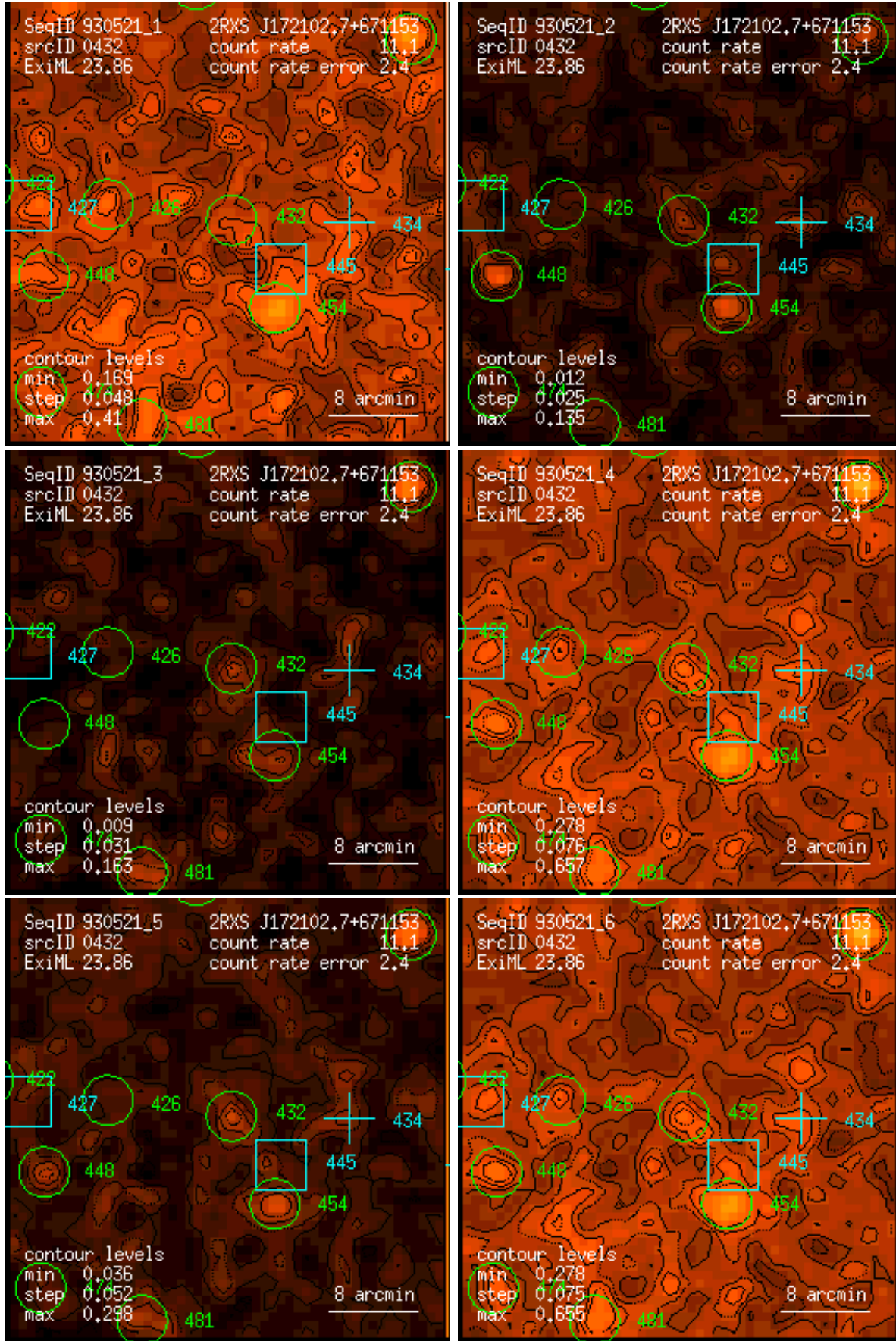
Figure 432: RASS 930521: detection 0432: band rate images, Gaussian filter: (1) PSPC channels 11 – 41, (2) 52 – 90, (3) 91 – 201, (4) 11 – 235, (5) 52 – 201, (6) 11 – 201. Broad band rates in counts/ks. Band rate contour levels in counts/ks/arcmin 2 .
