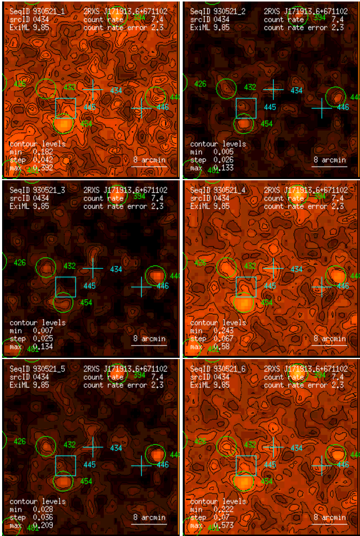
Figure 434: RASS 930521: detection 0434: band rate images, Gaussian filter: (1) PSPC channels 11 – 41, (2) 52 – 90, (3) 91 – 201, (4) 11 – 235, (5) 52 – 201, (6) 11 – 201. Broad band rates in counts/ks. Band rate contour levels in counts/ks/arcmin 2 .
