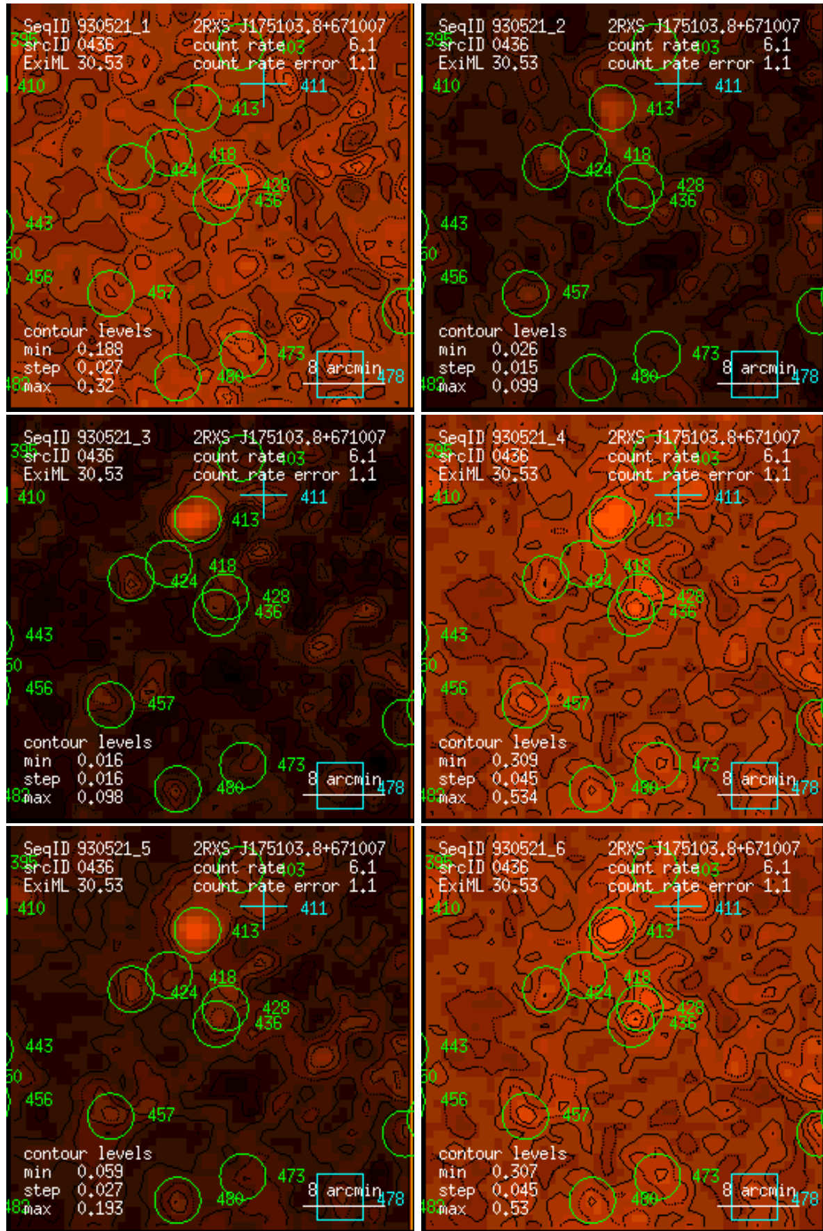
Figure 436: RASS 930521: detection 0436: band rate images, Gaussian filter: (1) PSPC channels 11 – 41, (2) 52 – 90, (3) 91 – 201, (4) 11 – 235, (5) 52 – 201, (6) 11 – 201. Broad band rates in counts/ks. Band rate contour levels in counts/ks/arcmin 2 .
