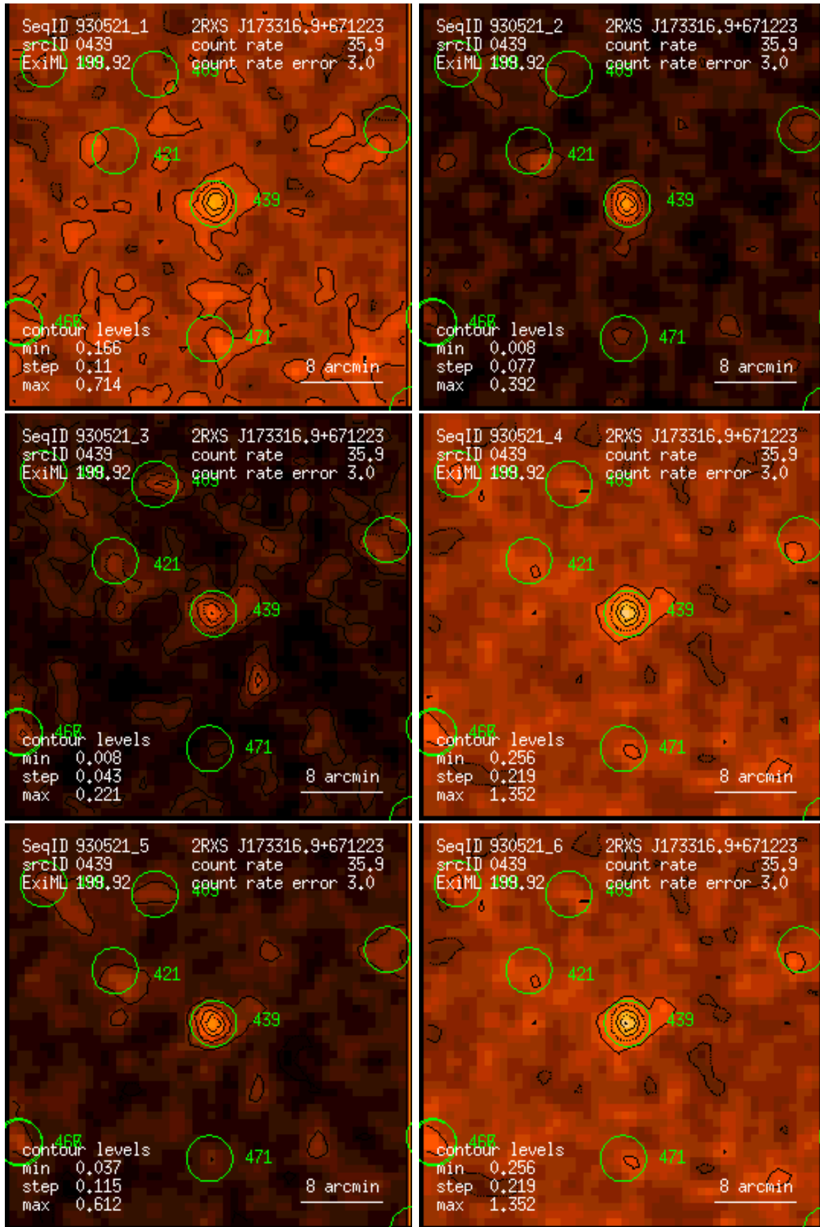
Figure 439: RASS 930521: detection 0439: band rate images, Gaussian filter: (1) PSPC channels 11 – 41, (2) 52 – 90, (3) 91 – 201, (4) 11 – 235, (5) 52 – 201, (6) 11 – 201. Broad band rates in counts/ks. Band rate contour levels in counts/ks/arcmin 2 .
