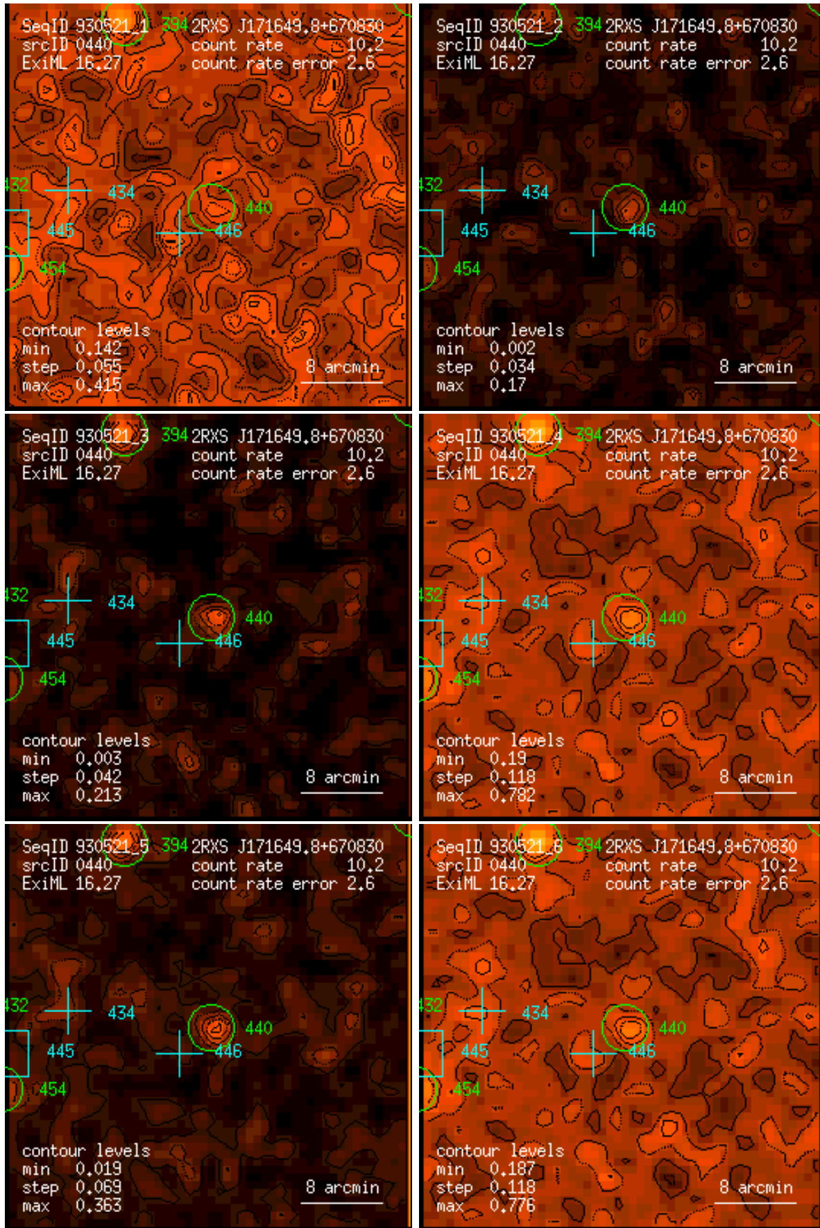
Figure 440: RASS 930521: detection 0440: band rate images, Gaussian filter: (1) PSPC channels 11 – 41, (2) 52 – 90, (3) 91 – 201, (4) 11 – 235, (5) 52 – 201, (6) 11 – 201. Broad band rates in counts/ks. Band rate contour levels in counts/ks/arcmin 2 .
