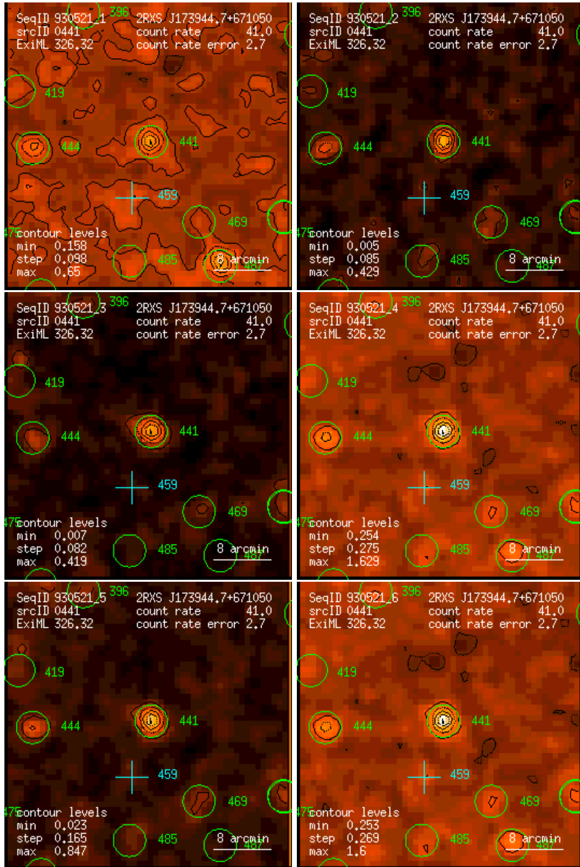
Figure 441: RASS 930521: detection 0441: band rate images, Gaussian filter: (1) PSPC channels 11 – 41, (2) 52 – 90, (3) 91 – 201, (4) 11 – 235, (5) 52 – 201, (6) 11 – 201. Broad band rates in counts/ks. Band rate contour levels in counts/ks/arcmin 2 .
