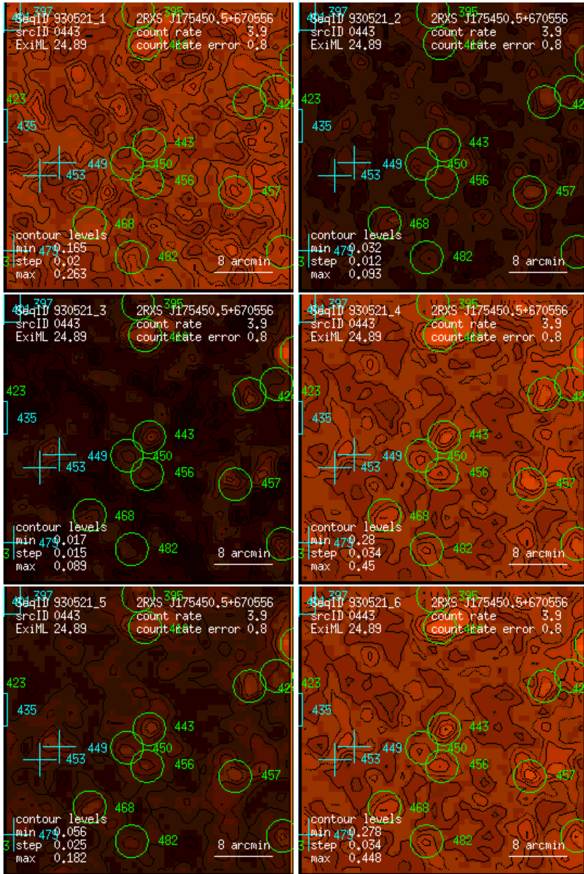
Figure 443: RASS 930521: detection 0443: band rate images, Gaussian filter: (1) PSPC channels 11 – 41, (2) 52 – 90, (3) 91 – 201, (4) 11 – 235, (5) 52 – 201, (6) 11 – 201. Broad band rates in counts/ks. Band rate contour levels in counts/ks/arcmin 2 .
