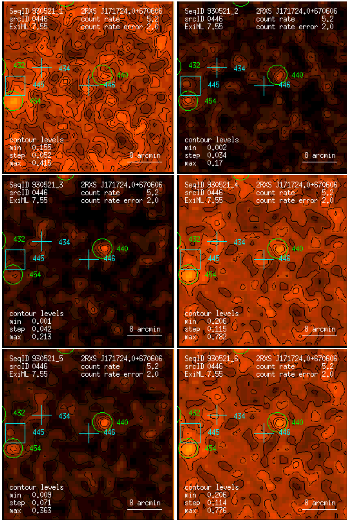
Figure 446: RASS 930521: detection 0446: band rate images, Gaussian filter: (1) PSPC channels 11 – 41, (2) 52 – 90, (3) 91 – 201, (4) 11 – 235, (5) 52 – 201, (6) 11 – 201. Broad band rates in counts/ks. Band rate contour levels in counts/ks/arcmin 2 .
