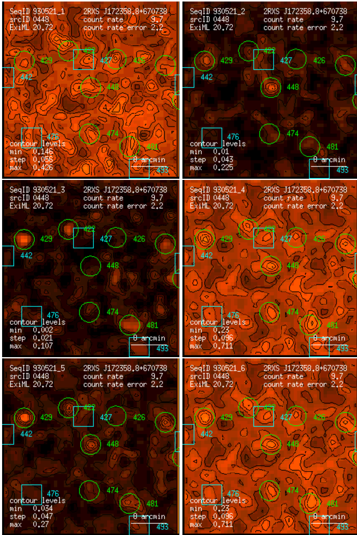
Figure 448: RASS 930521: detection 0448: band rate images, Gaussian filter: (1) PSPC channels 11 – 41, (2) 52 – 90, (3) 91 – 201, (4) 11 – 235, (5) 52 – 201, (6) 11 – 201. Broad band rates in counts/ks. Band rate contour levels in counts/ks/arcmin 2 .
