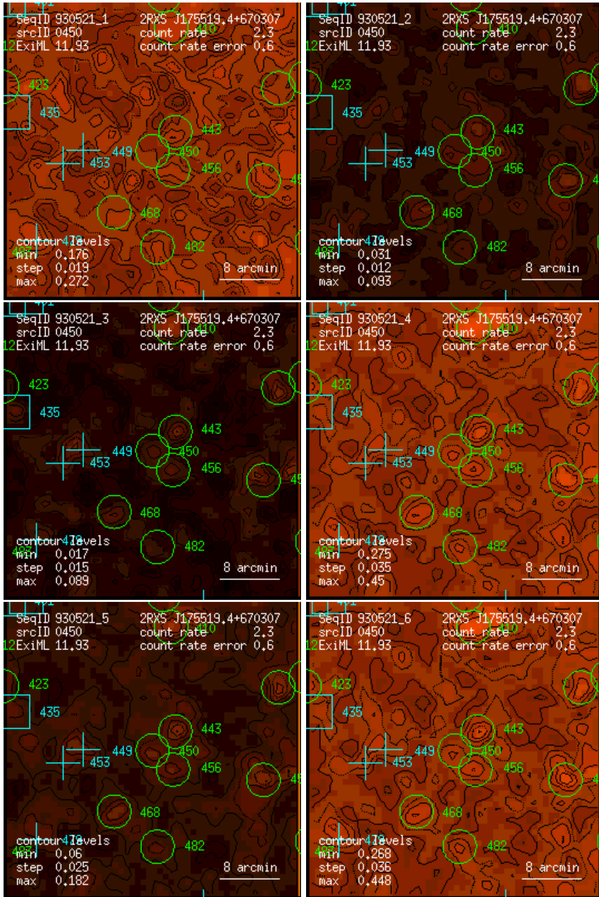
Figure 450: RASS 930521: detection 0450: band rate images, Gaussian filter: (1) PSPC channels 11 – 41, (2) 52 – 90, (3) 91 – 201, (4) 11 – 235, (5) 52 – 201, (6) 11 – 201. Broad band rates in counts/ks. Band rate contour levels in counts/ks/arcmin 2 .
