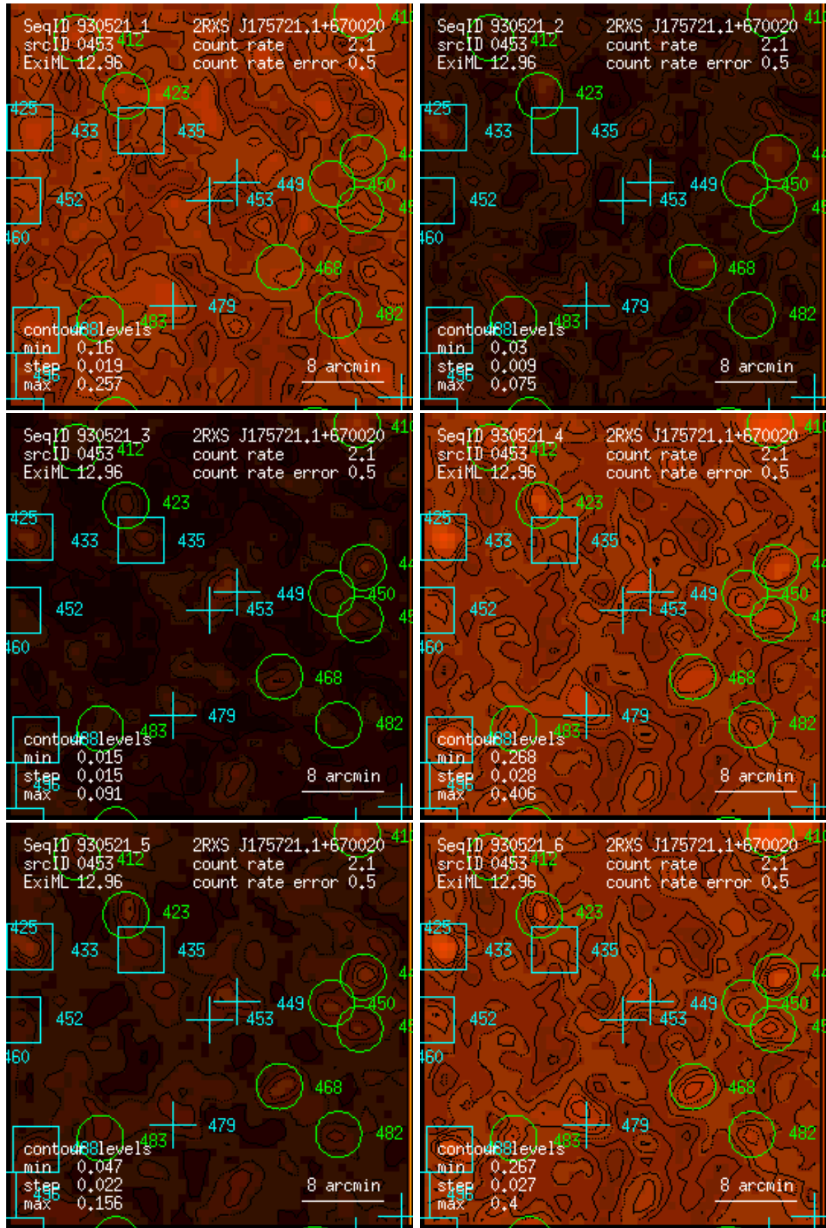
Figure 453: RASS 930521: detection 0453: band rate images, Gaussian filter: (1) PSPC channels 11 – 41, (2) 52 – 90, (3) 91 – 201, (4) 11 – 235, (5) 52 – 201, (6) 11 – 201. Broad band rates in counts/ks. Band rate contour levels in counts/ks/arcmin 2 .
