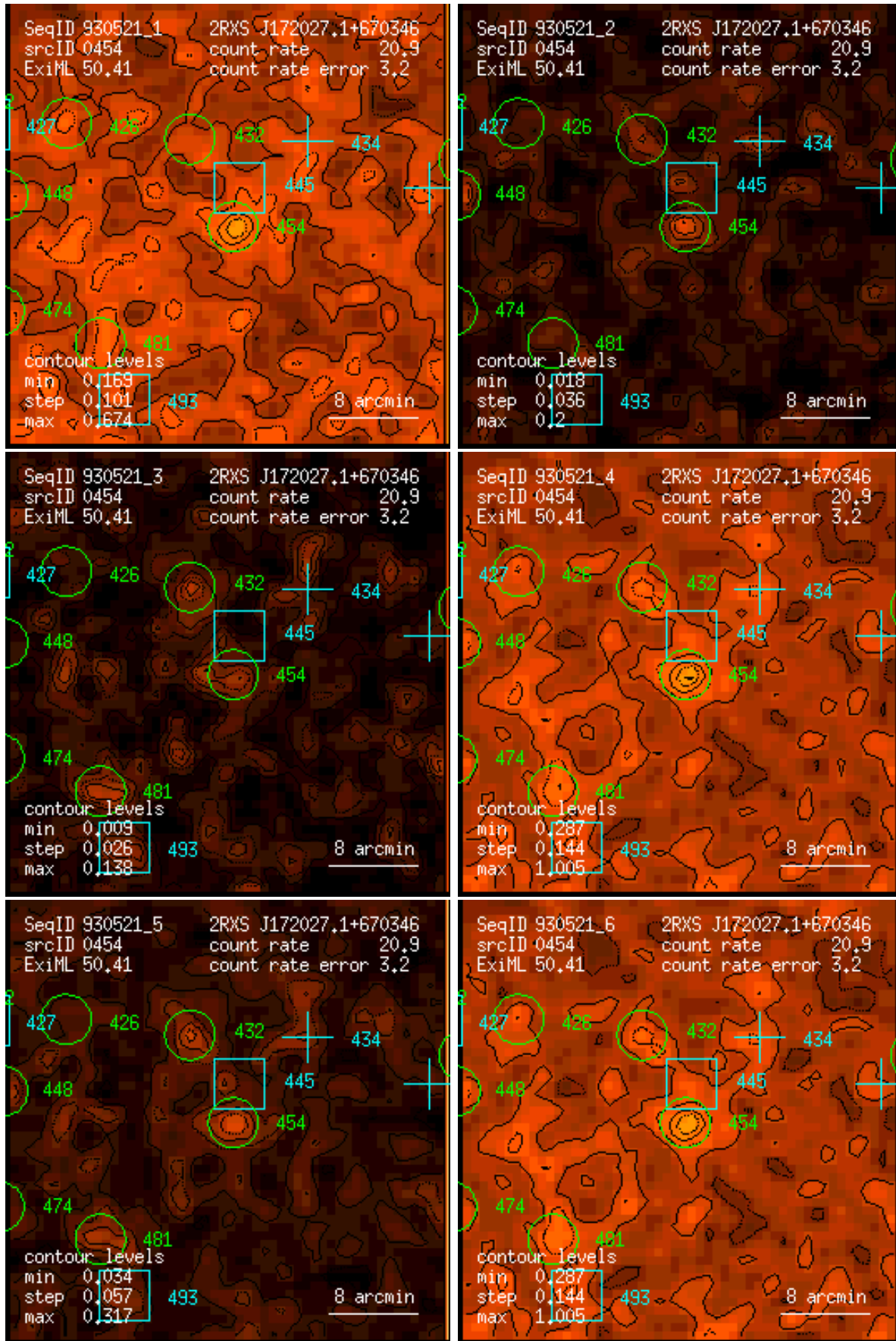
Figure 454: RASS 930521: detection 0454: band rate images, Gaussian filter: (1) PSPC channels 11 – 41, (2) 52 – 90, (3) 91 – 201, (4) 11 – 235, (5) 52 – 201, (6) 11 – 201. Broad band rates in counts/ks. Band rate contour levels in counts/ks/arcmin 2 .
