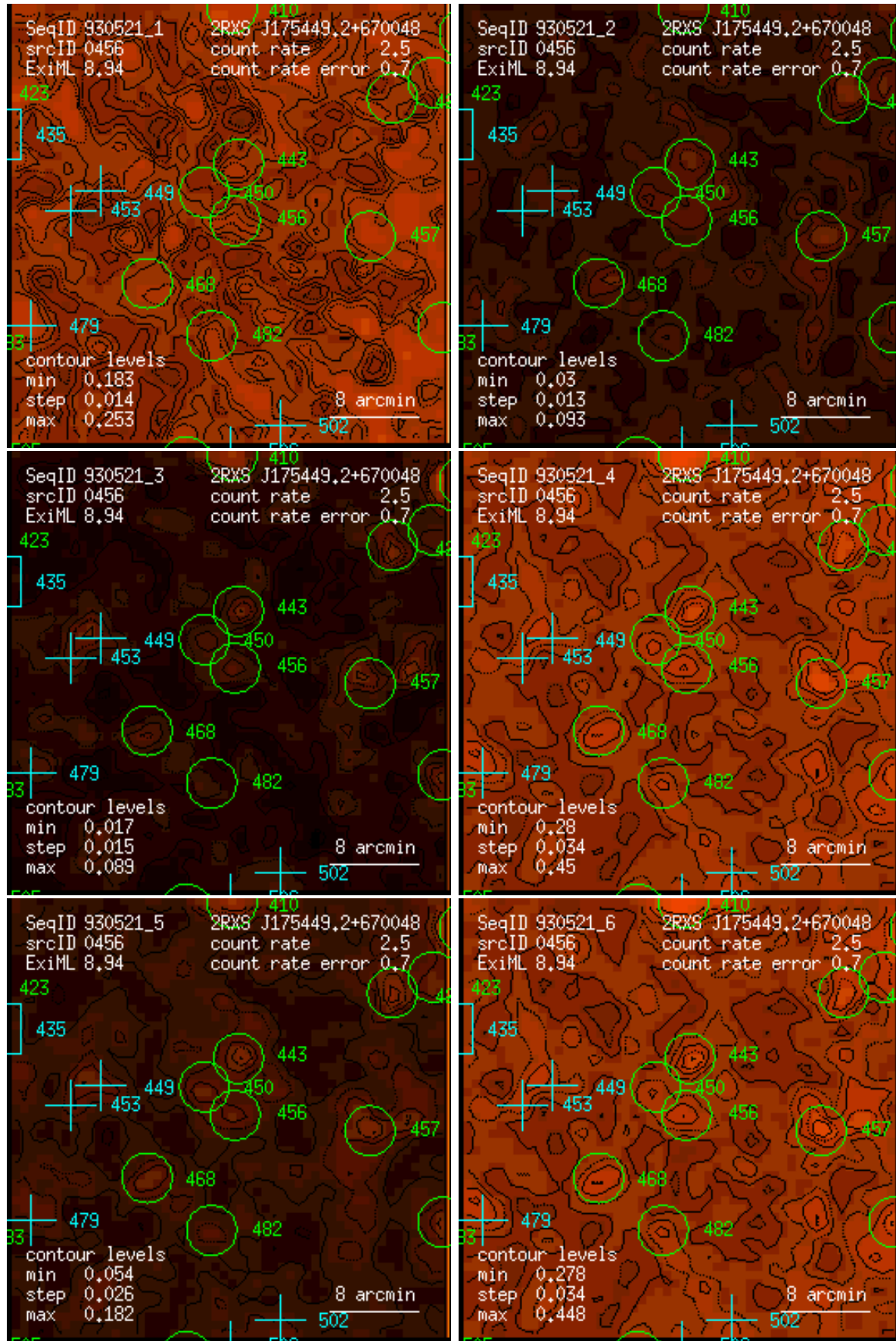
Figure 456: RASS 930521: detection 0456: band rate images, Gaussian filter: (1) PSPC channels 11 – 41, (2) 52 – 90, (3) 91 – 201, (4) 11 – 235, (5) 52 – 201, (6) 11 – 201. Broad band rates in counts/ks. Band rate contour levels in counts/ks/arcmin 2 .
