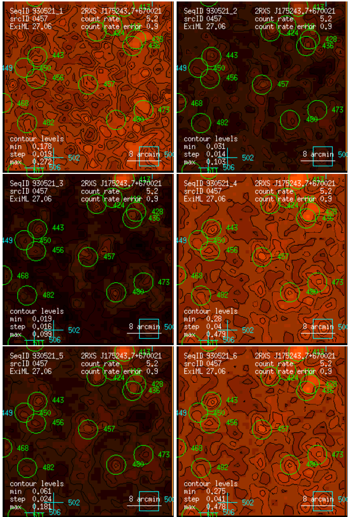
Figure 457: RASS 930521: detection 0457: band rate images, Gaussian filter: (1) PSPC channels 11 – 41, (2) 52 – 90, (3) 91 – 201, (4) 11 – 235, (5) 52 – 201, (6) 11 – 201. Broad band rates in counts/ks. Band rate contour levels in counts/ks/arcmin 2 .
