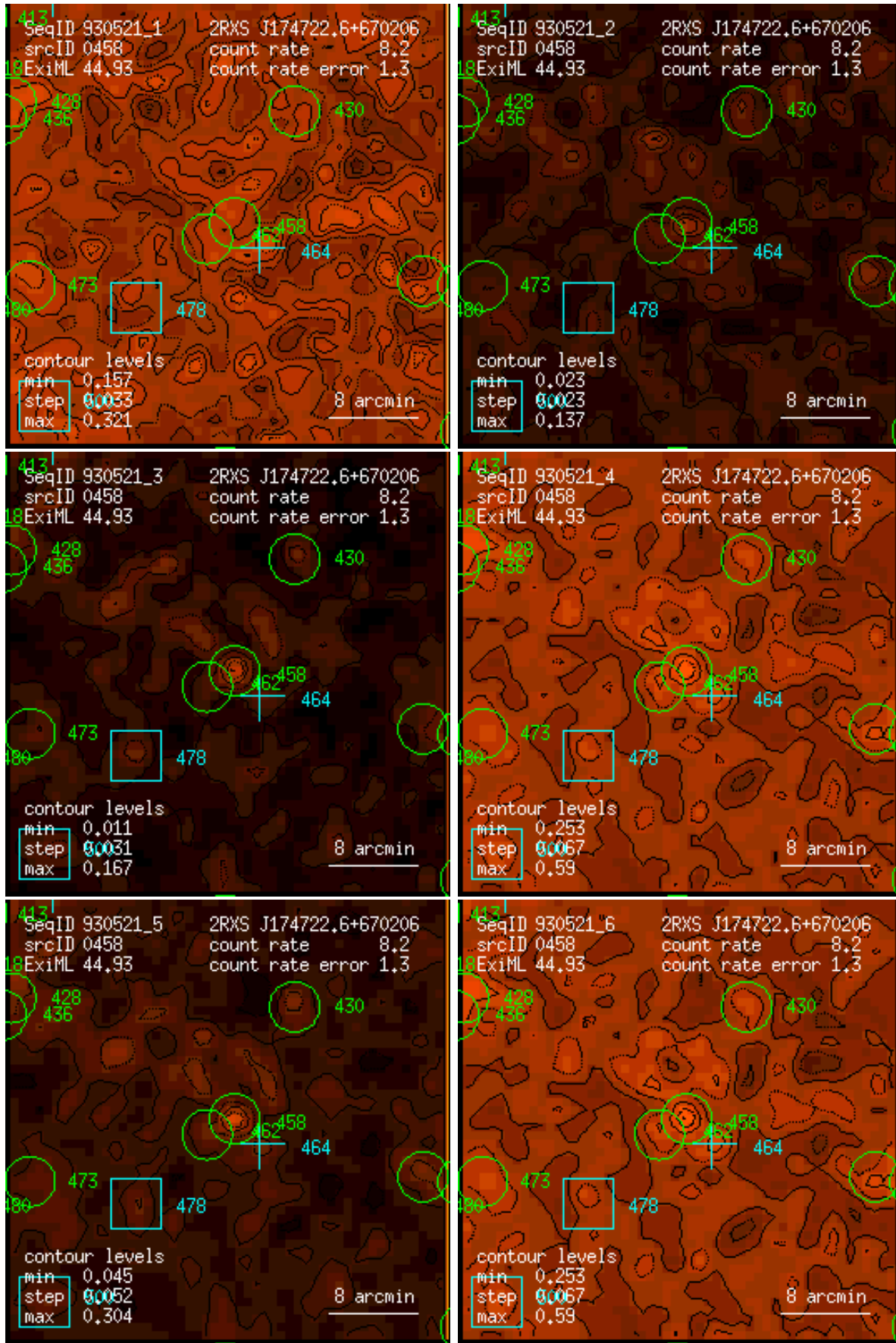
Figure 458: RASS 930521: detection 0458: band rate images, Gaussian filter: (1) PSPC channels 11 – 41, (2) 52 – 90, (3) 91 – 201, (4) 11 – 235, (5) 52 – 201, (6) 11 – 201. Broad band rates in counts/ks. Band rate contour levels in counts/ks/arcmin 2 .
