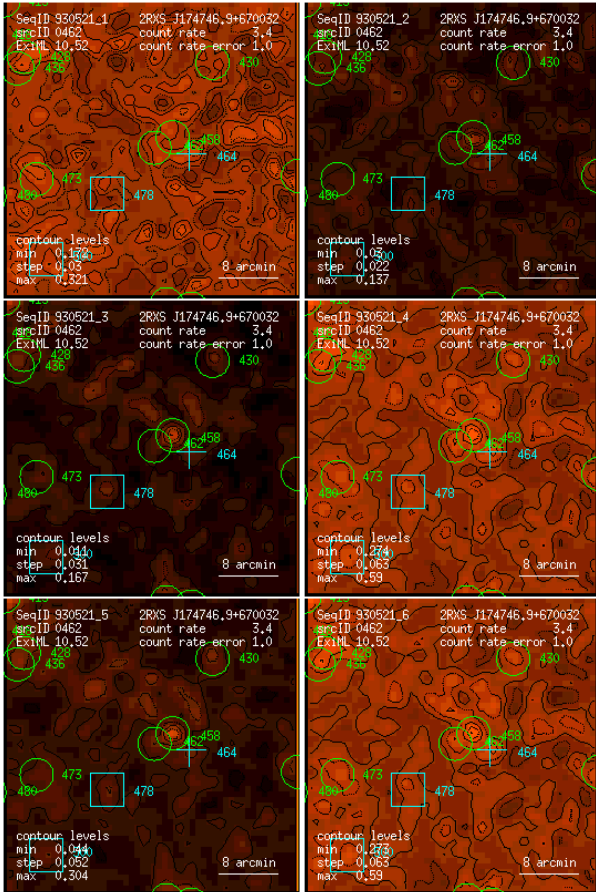
Figure 462: RASS 930521: detection 0462: band rate images, Gaussian filter: (1) PSPC channels 11 – 41, (2) 52 – 90, (3) 91 – 201, (4) 11 – 235, (5) 52 – 201, (6) 11 – 201. Broad band rates in counts/ks. Band rate contour levels in counts/ks/arcmin 2 .
