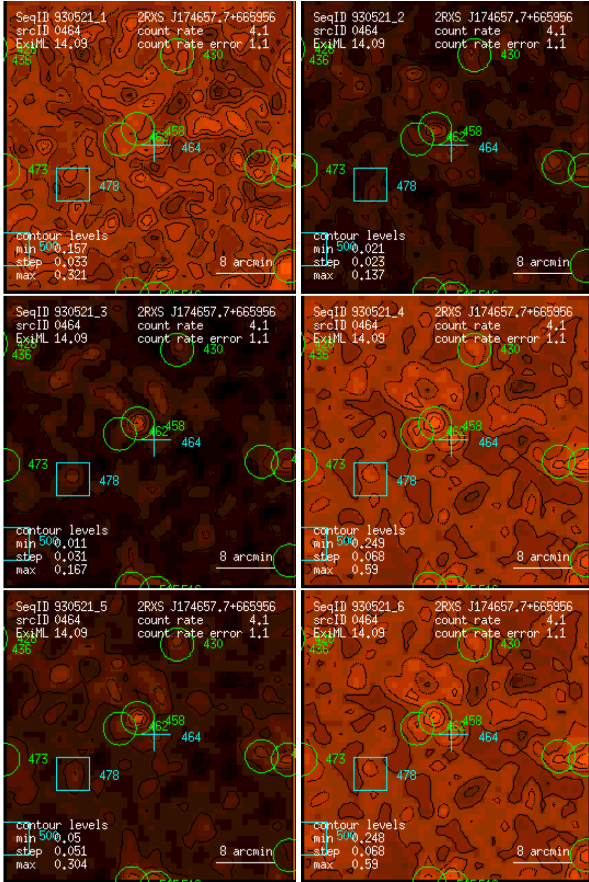
Figure 464: RASS 930521: detection 0464: band rate images, Gaussian filter: (1) PSPC channels 11 – 41, (2) 52 – 90, (3) 91 – 201, (4) 11 – 235, (5) 52 – 201, (6) 11 – 201. Broad band rates in counts/ks. Band rate contour levels in counts/ks/arcmin 2 .
