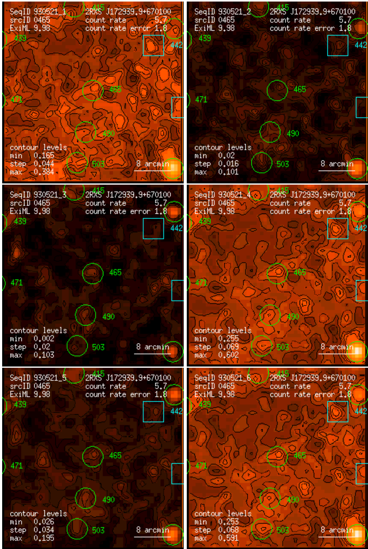
Figure 465: RASS 930521: detection 0465: band rate images, Gaussian filter: (1) PSPC channels 11 – 41, (2) 52 – 90, (3) 91 – 201, (4) 11 – 235, (5) 52 – 201, (6) 11 – 201. Broad band rates in counts/ks. Band rate contour levels in counts/ks/arcmin 2 .
