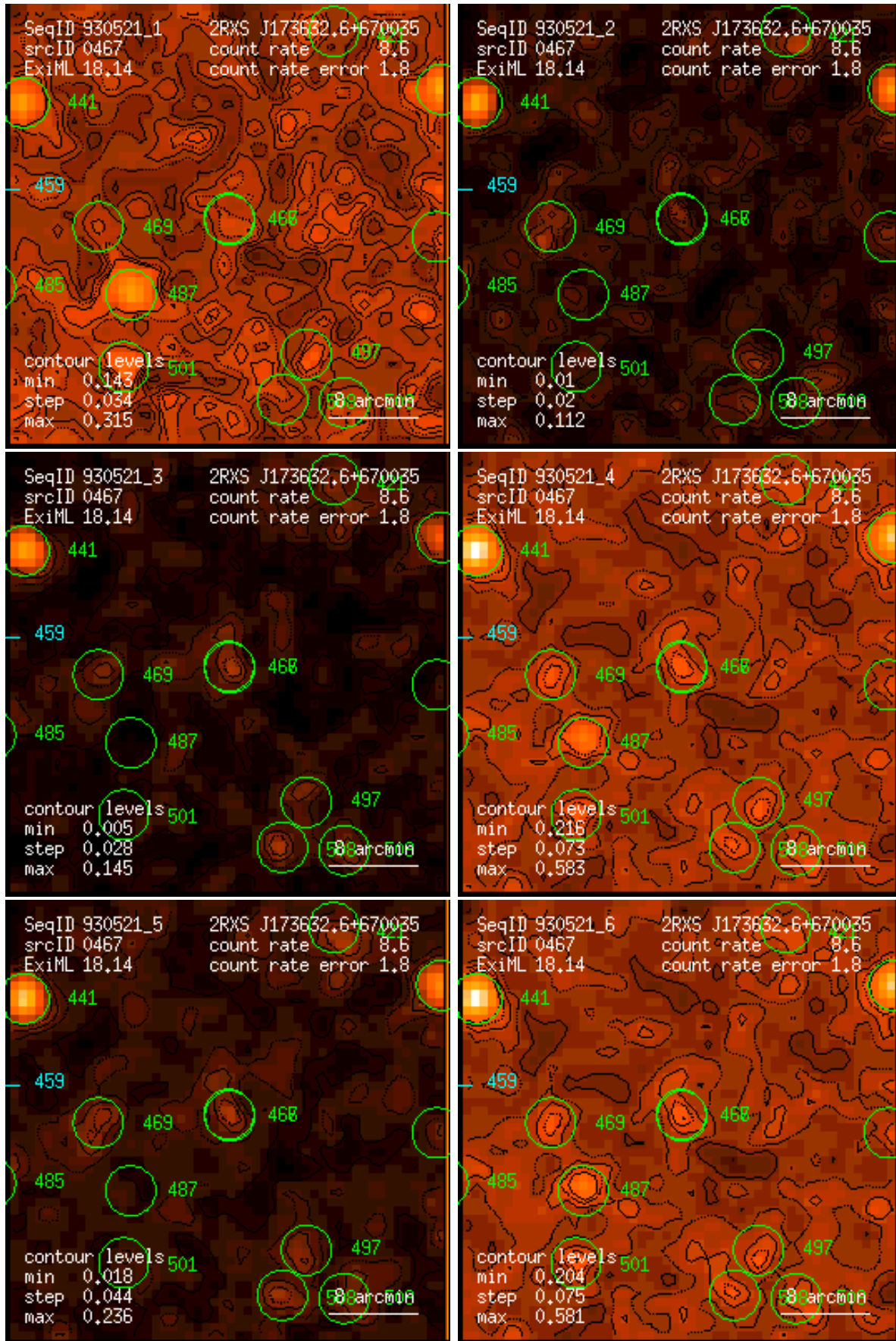
Figure 467: RASS 930521: detection 0467: band rate images, Gaussian filter: (1) PSPC channels 11 – 41, (2) 52 – 90, (3) 91 – 201, (4) 11 – 235, (5) 52 – 201, (6) 11 – 201. Broad band rates in counts/ks. Band rate contour levels in counts/ks/arcmin 2 .
