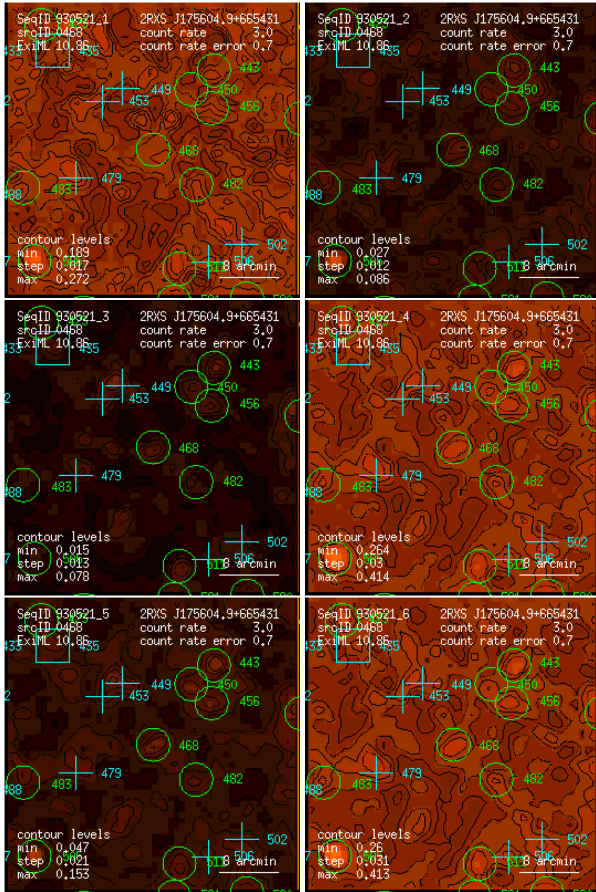
Figure 468: RASS 930521: detection 0468: band rate images, Gaussian filter: (1) PSPC channels 11 – 41, (2) 52 – 90, (3) 91 – 201, (4) 11 – 235, (5) 52 – 201, (6) 11 – 201. Broad band rates in counts/ks. Band rate contour levels in counts/ks/arcmin 2 .
