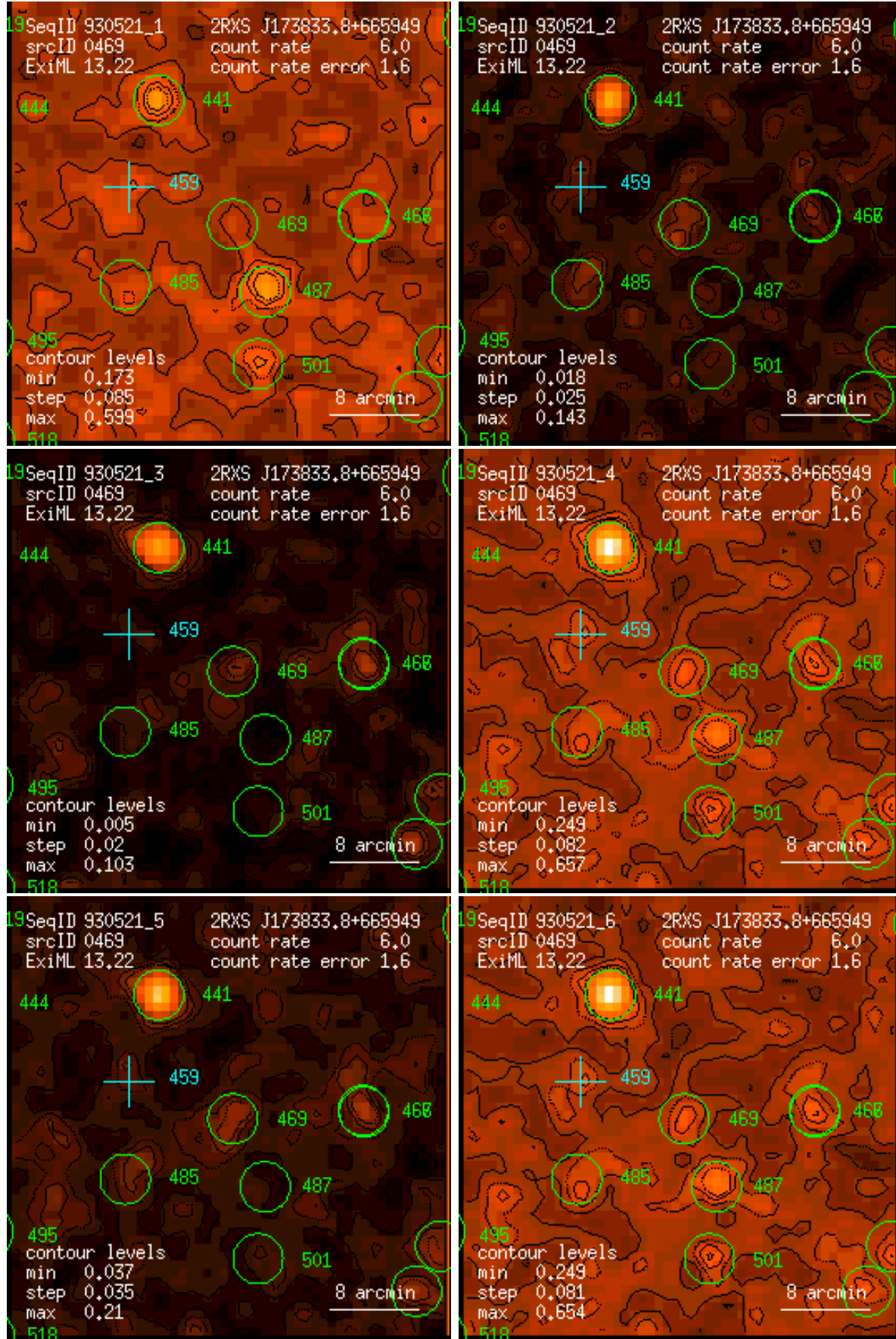
Figure 469: RASS 930521: detection 0469: band rate images, Gaussian filter: (1) PSPC channels 11 – 41, (2) 52 – 90, (3) 91 – 201, (4) 11 – 235, (5) 52 – 201, (6) 11 – 201. Broad band rates in counts/ks. Band rate contour levels in counts/ks/arcmin 2 .
