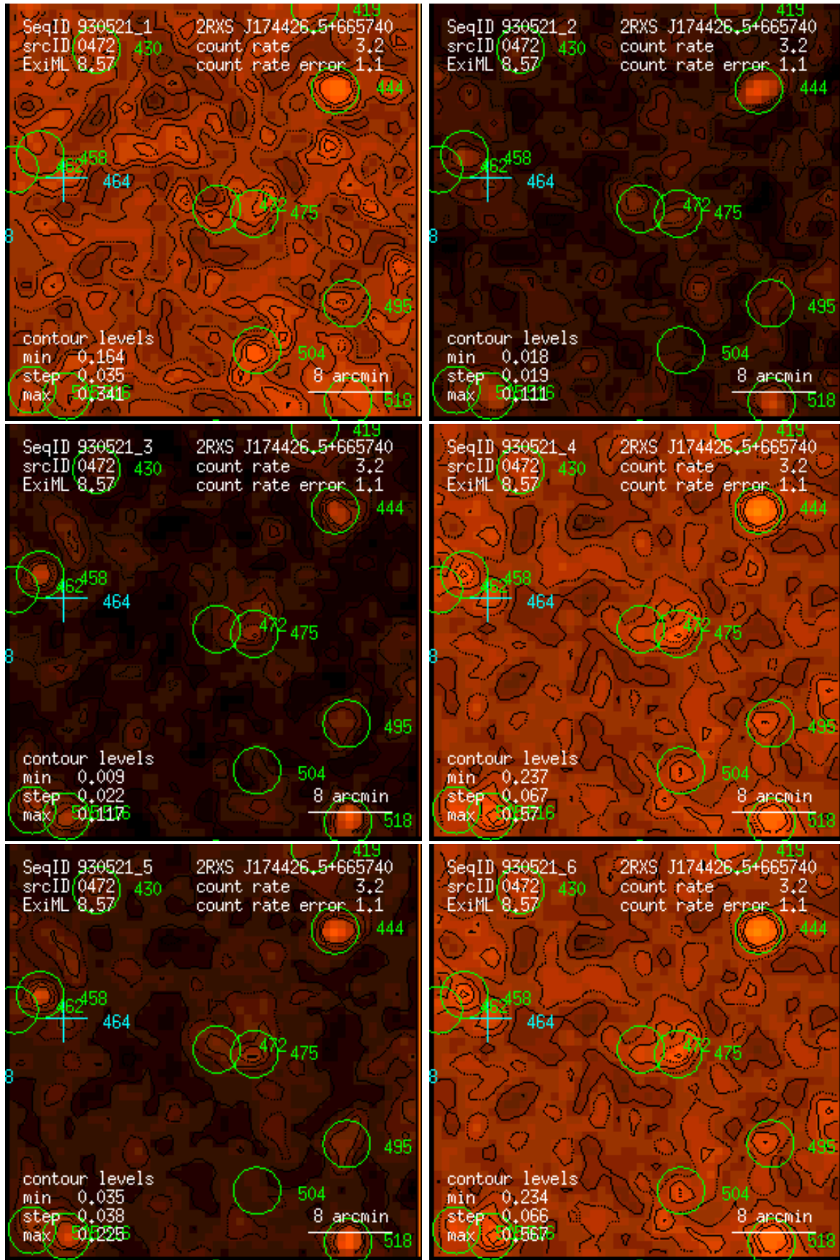
Figure 472: RASS 930521: detection 0472: band rate images, Gaussian filter: (1) PSPC channels 11 – 41, (2) 52 – 90, (3) 91 – 201, (4) 11 – 235, (5) 52 – 201, (6) 11 – 201. Broad band rates in counts/ks. Band rate contour levels in counts/ks/arcmin 2 .
