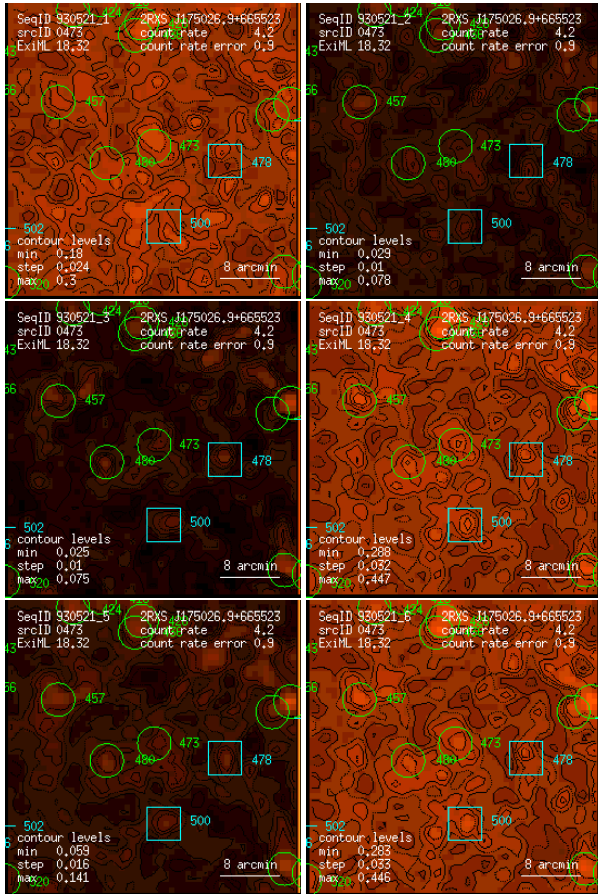
Figure 473: RASS 930521: detection 0473: band rate images, Gaussian filter: (1) PSPC channels 11 – 41, (2) 52 – 90, (3) 91 – 201, (4) 11 – 235, (5) 52 – 201, (6) 11 – 201. Broad band rates in counts/ks. Band rate contour levels in counts/ks/arcmin 2 .
