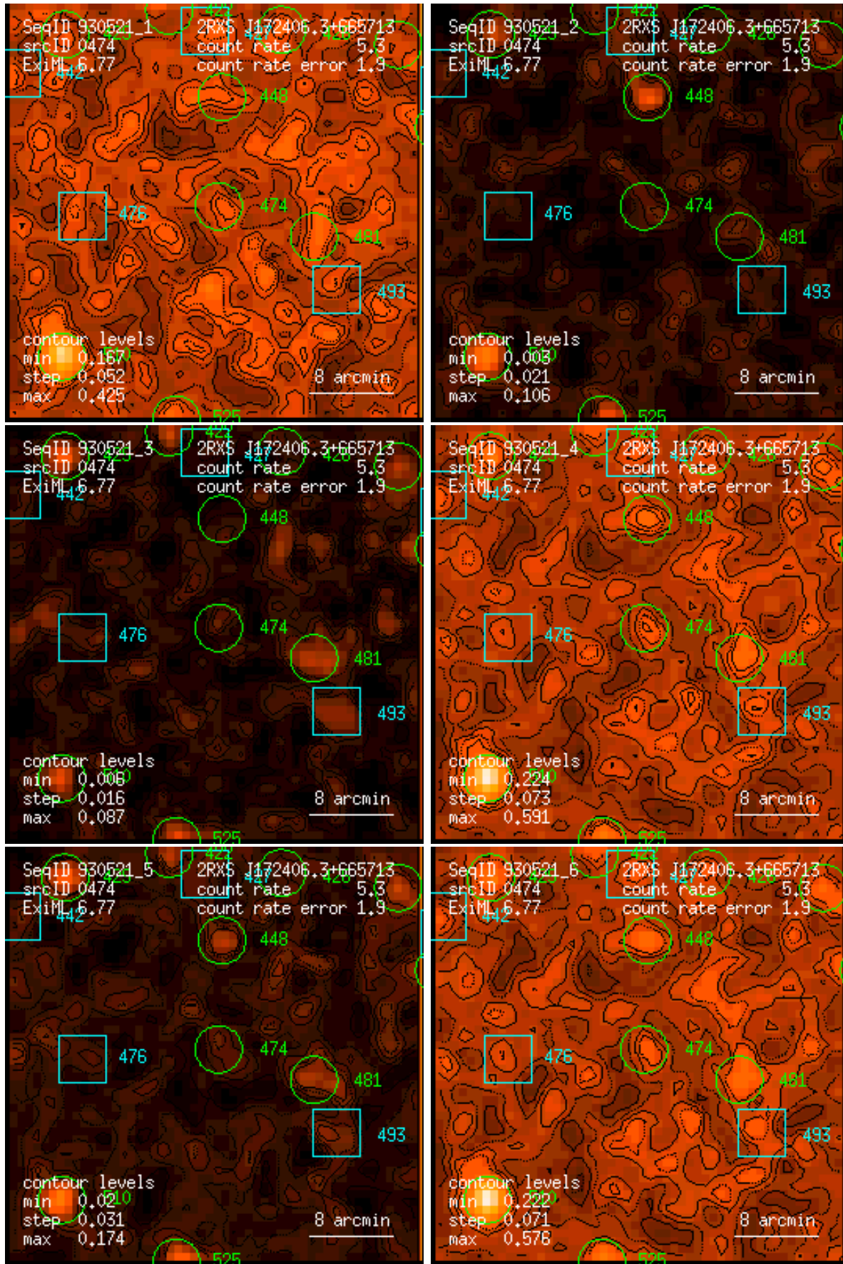
Figure 474: RASS 930521: detection 0474: band rate images, Gaussian filter: (1) PSPC channels 11 – 41, (2) 52 – 90, (3) 91 – 201, (4) 11 – 235, (5) 52 – 201, (6) 11 – 201. Broad band rates in counts/ks. Band rate contour levels in counts/ks/arcmin 2 .
