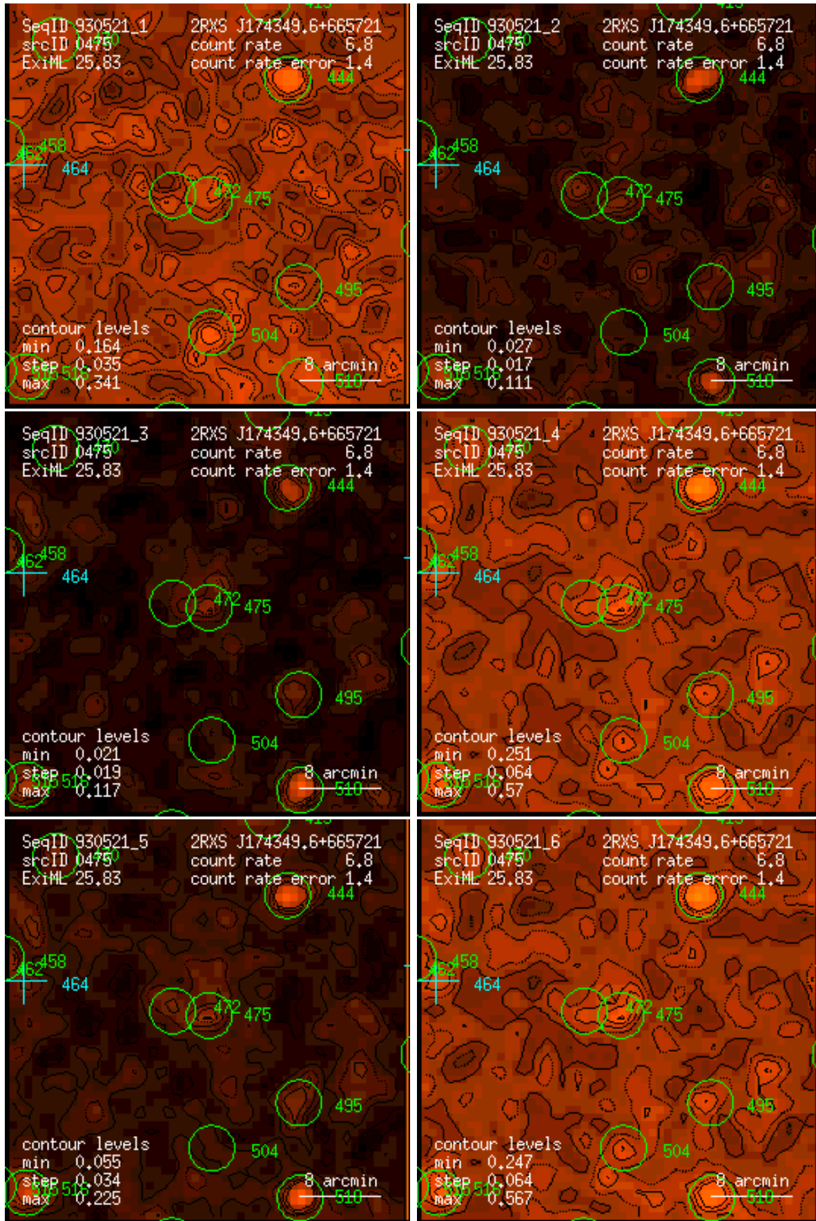
Figure 475: RASS 930521: detection 0475: band rate images, Gaussian filter: (1) PSPC channels 11 – 41, (2) 52 – 90, (3) 91 – 201, (4) 11 – 235, (5) 52 – 201, (6) 11 – 201. Broad band rates in counts/ks. Band rate contour levels in counts/ks/arcmin 2 .
