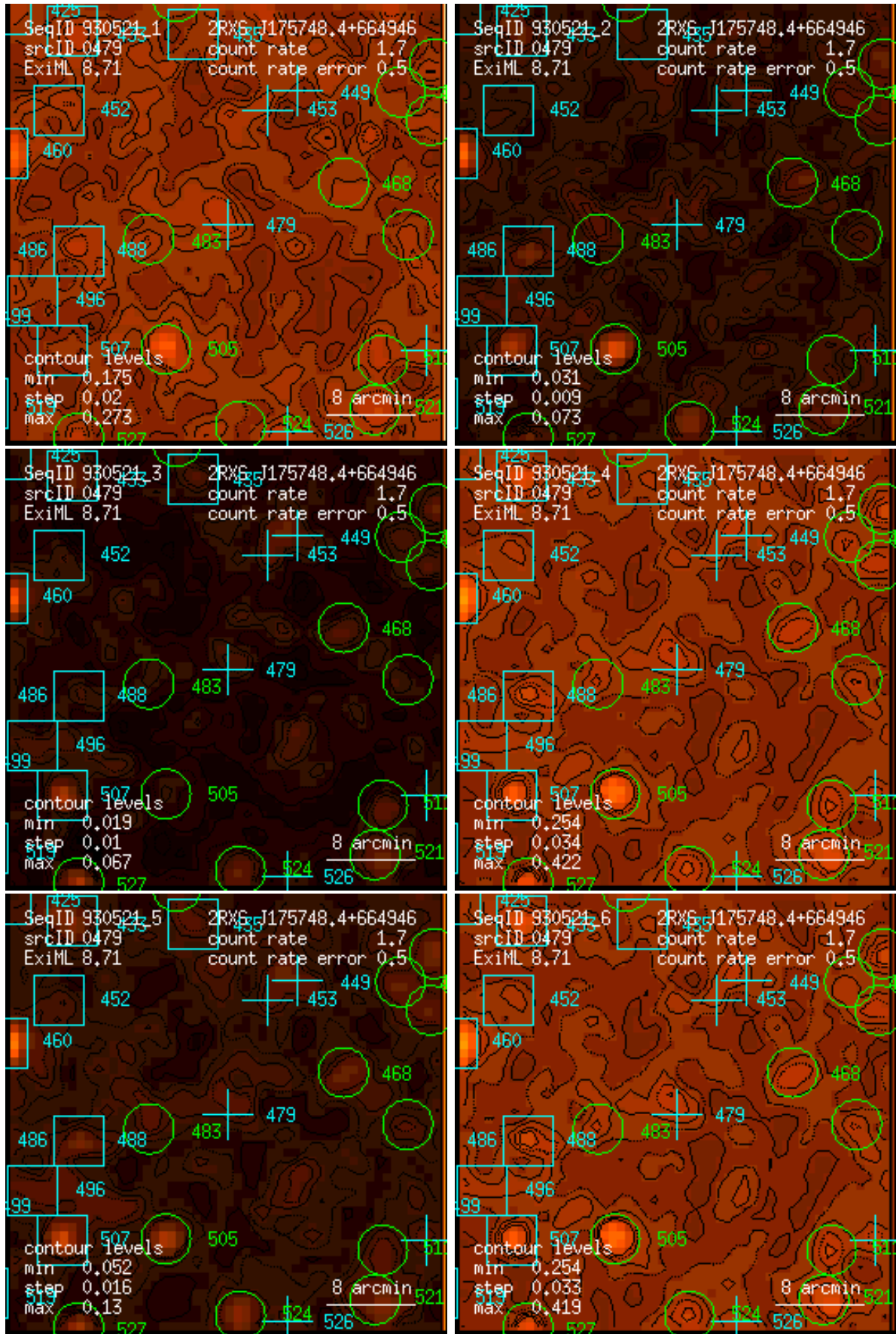
Figure 479: RASS 930521: detection 0479: band rate images, Gaussian filter: (1) PSPC channels 11 – 41, (2) 52 – 90, (3) 91 – 201, (4) 11 – 235, (5) 52 – 201, (6) 11 – 201. Broad band rates in counts/ks. Band rate contour levels in counts/ks/arcmin 2 .
