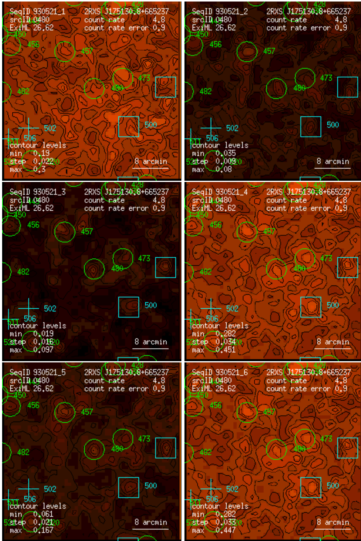
Figure 480: RASS 930521: detection 0480: band rate images, Gaussian filter: (1) PSPC channels 11 – 41, (2) 52 – 90, (3) 91 – 201, (4) 11 – 235, (5) 52 – 201, (6) 11 – 201. Broad band rates in counts/ks. Band rate contour levels in counts/ks/arcmin 2 .
