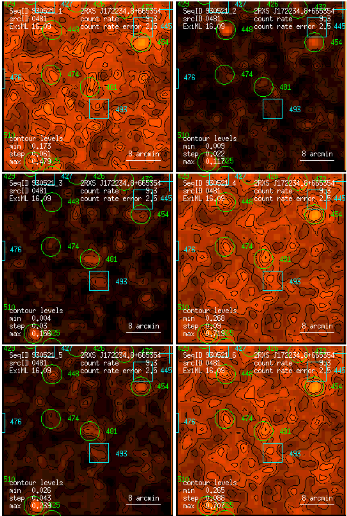
Figure 481: RASS 930521: detection 0481: band rate images, Gaussian filter: (1) PSPC channels 11 – 41, (2) 52 – 90, (3) 91 – 201, (4) 11 – 235, (5) 52 – 201, (6) 11 – 201. Broad band rates in counts/ks. Band rate contour levels in counts/ks/arcmin 2 .
