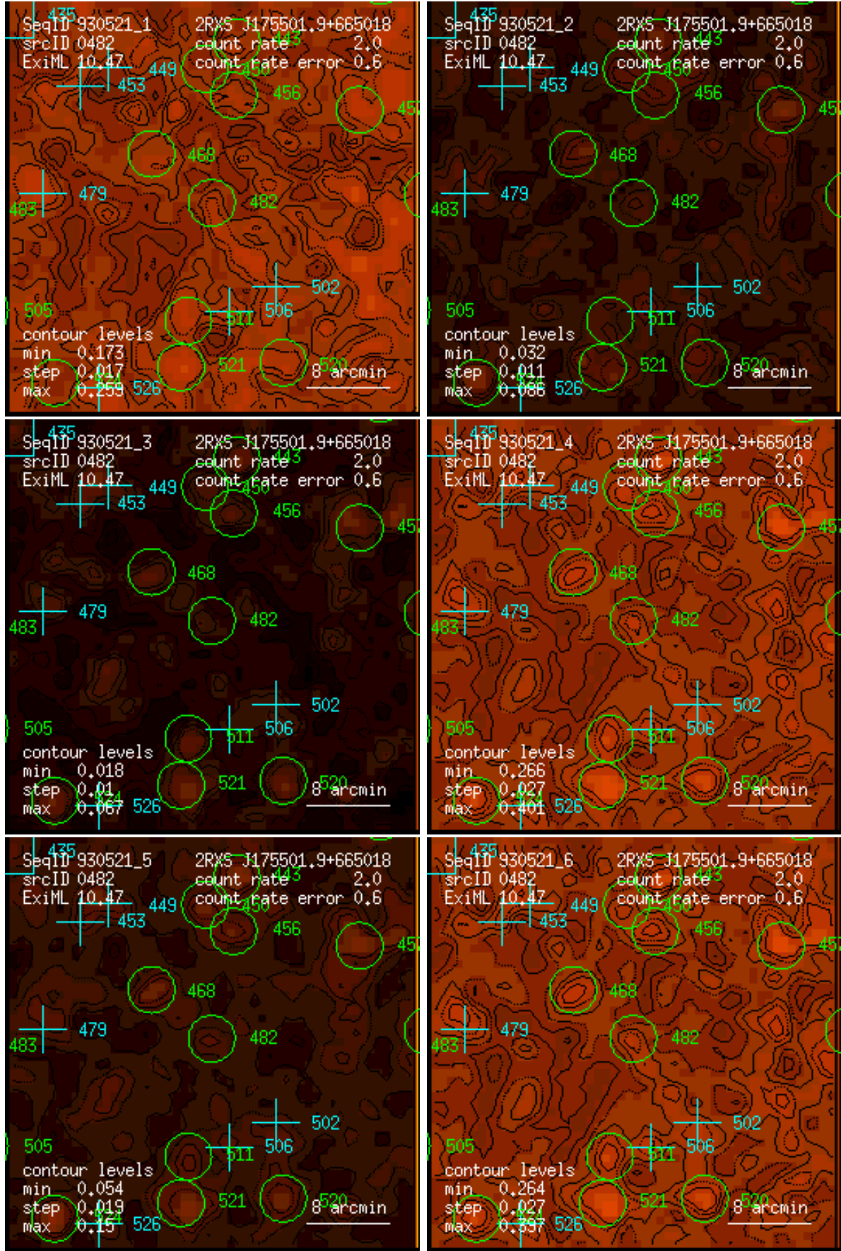
Figure 482: RASS 930521: detection 0482: band rate images, Gaussian filter: (1) PSPC channels 11 – 41, (2) 52 – 90, (3) 91 – 201, (4) 11 – 235, (5) 52 – 201, (6) 11 – 201. Broad band rates in counts/ks. Band rate contour levels in counts/ks/arcmin 2 .
