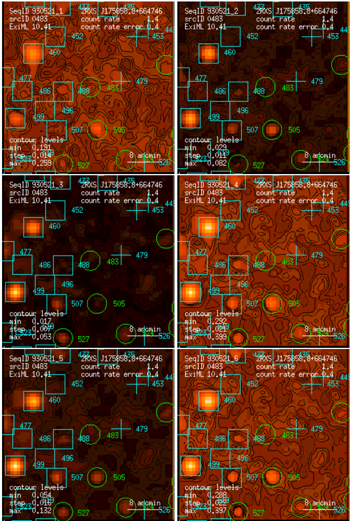
Figure 483: RASS 930521: detection 0483: band rate images, Gaussian filter: (1) PSPC channels 11 – 41, (2) 52 – 90, (3) 91 – 201, (4) 11 – 235, (5) 52 – 201, (6) 11 – 201. Broad band rates in counts/ks. Band rate contour levels in counts/ks/arcmin 2 .
