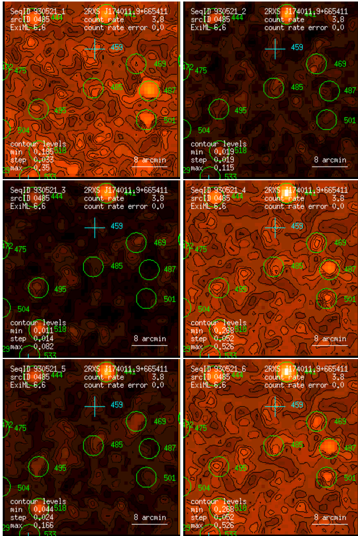
Figure 485: RASS 930521: detection 0485: band rate images, Gaussian filter: (1) PSPC channels 11 – 41, (2) 52 – 90, (3) 91 – 201, (4) 11 – 235, (5) 52 – 201, (6) 11 – 201. Broad band rates in counts/ks. Band rate contour levels in counts/ks/arcmin 2 .
