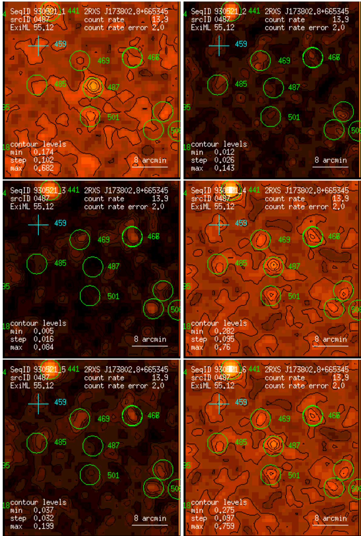
Figure 487: RASS 930521: detection 0487: band rate images, Gaussian filter: (1) PSPC channels 11 – 41, (2) 52 – 90, (3) 91 – 201, (4) 11 – 235, (5) 52 – 201, (6) 11 – 201. Broad band rates in counts/ks. Band rate contour levels in counts/ks/arcmin 2 .
