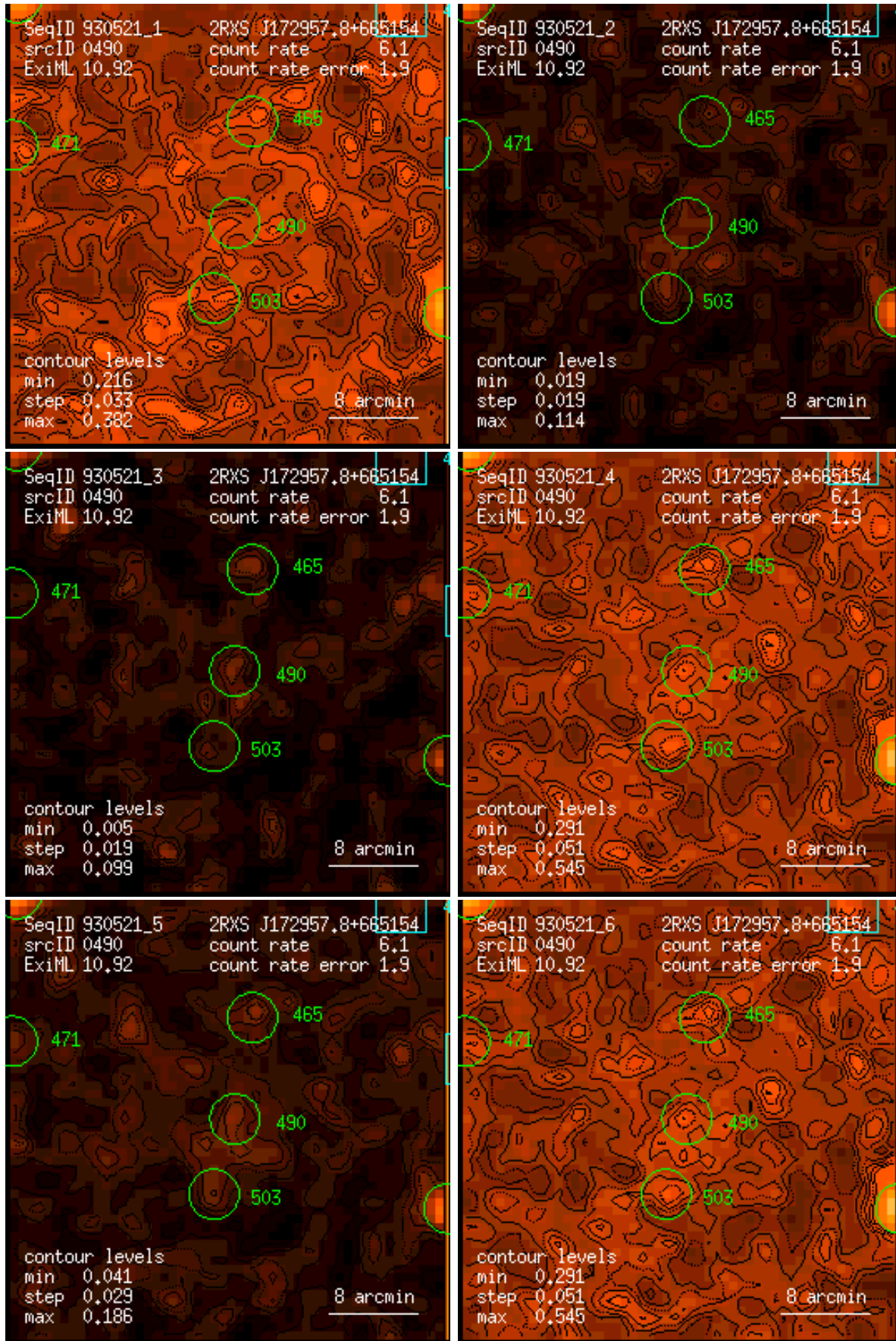
Figure 490: RASS 930521: detection 0490: band rate images, Gaussian filter: (1) PSPC channels 11 – 41, (2) 52 – 90, (3) 91 – 201, (4) 11 – 235, (5) 52 – 201, (6) 11 – 201. Broad band rates in counts/ks. Band rate contour levels in counts/ks/arcmin 2 .
