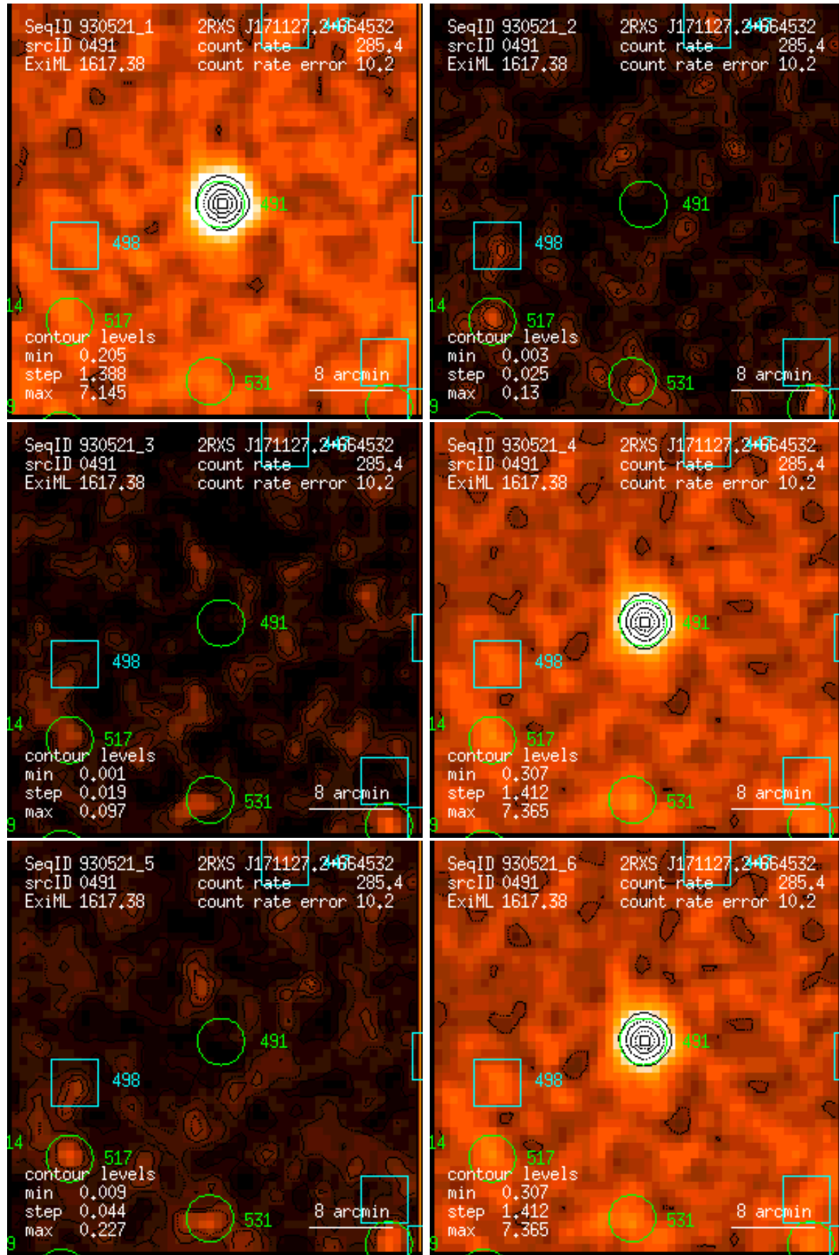
Figure 491: RASS 930521: detection 0491: band rate images, Gaussian filter: (1) PSPC channels 11 – 41, (2) 52 – 90, (3) 91 – 201, (4) 11 – 235, (5) 52 – 201, (6) 11 – 201. Broad band rates in counts/ks. Band rate contour levels in counts/ks/arcmin 2 .
