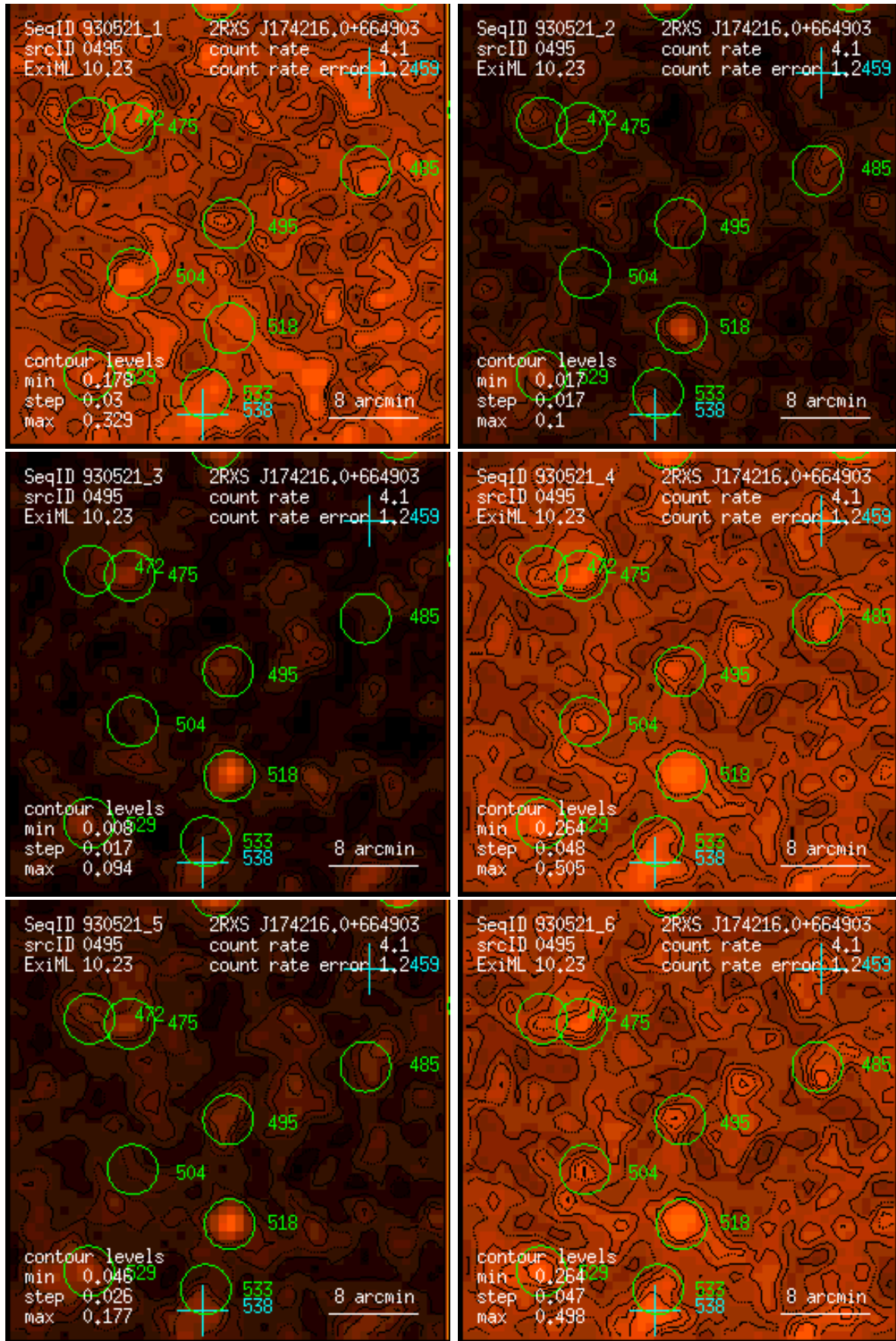
Figure 495: RASS 930521: detection 0495: band rate images, Gaussian filter: (1) PSPC channels 11 – 41, (2) 52 – 90, (3) 91 – 201, (4) 11 – 235, (5) 52 – 201, (6) 11 – 201. Broad band rates in counts/ks. Band rate contour levels in counts/ks/arcmin 2 .
