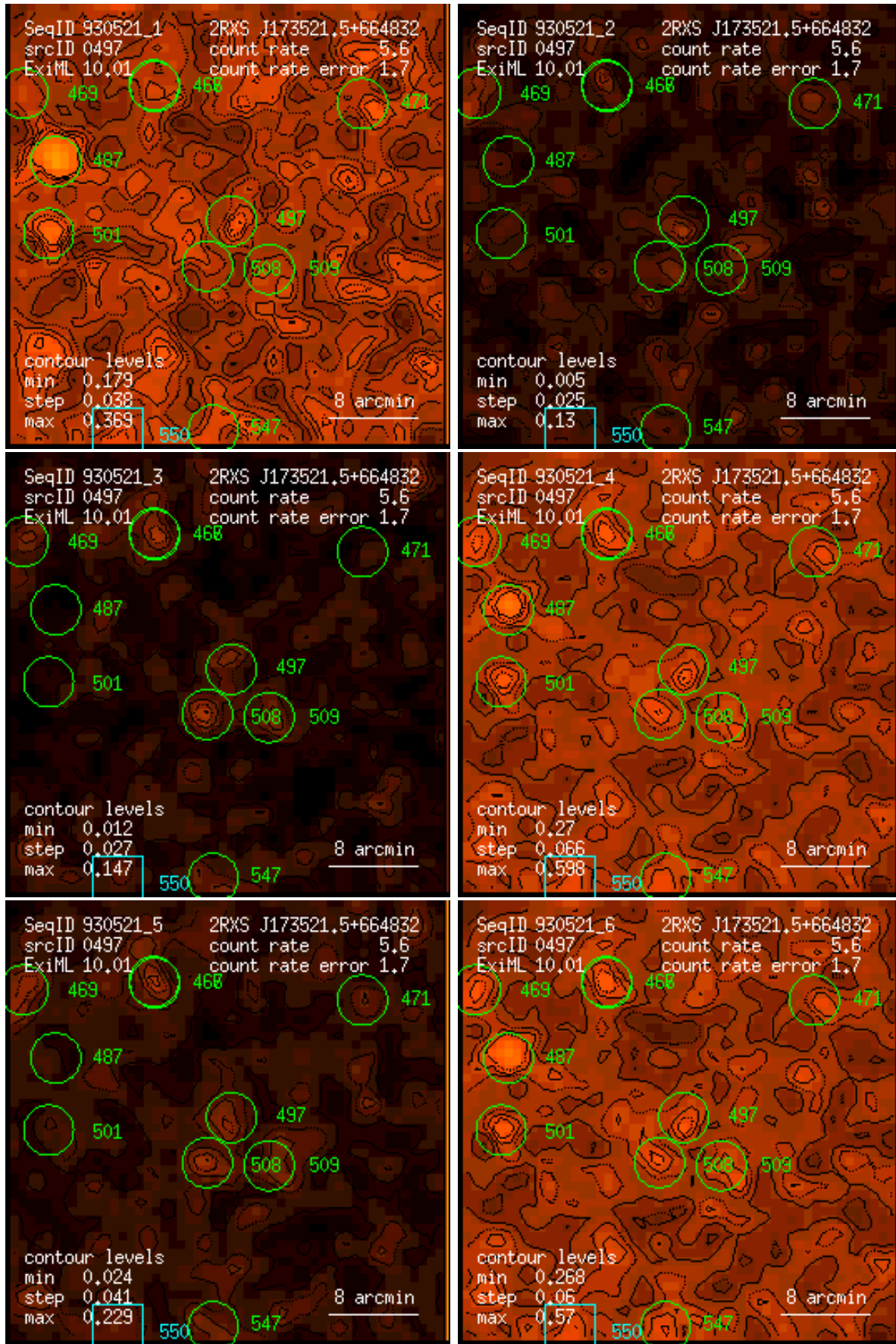
Figure 497: RASS 930521: detection 0497: band rate images, Gaussian filter: (1) PSPC channels 11 – 41, (2) 52 – 90, (3) 91 – 201, (4) 11 – 235, (5) 52 – 201, (6) 11 – 201. Broad band rates in counts/ks. Band rate contour levels in counts/ks/arcmin 2 .
