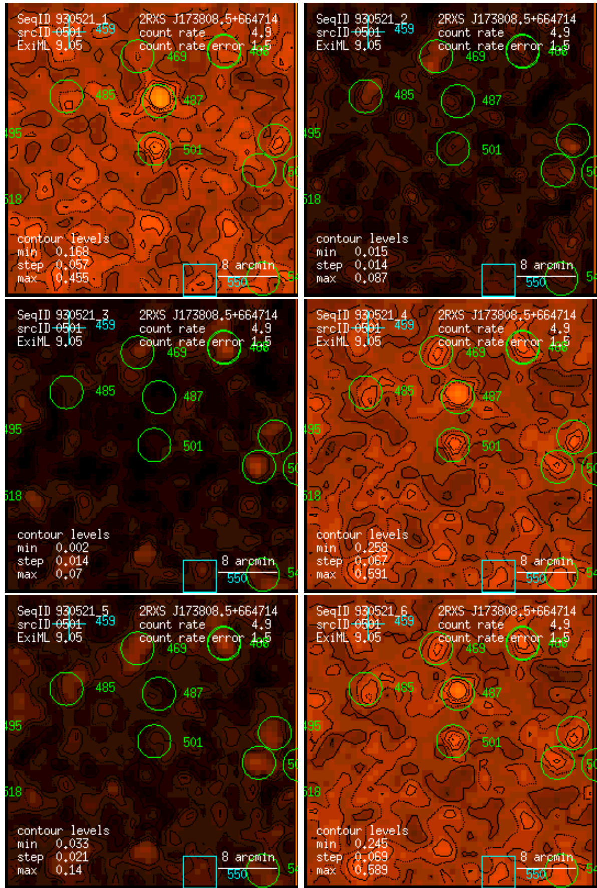
Figure 501: RASS 930521: detection 0501: band rate images, Gaussian filter: (1) PSPC channels 11 – 41, (2) 52 – 90, (3) 91 – 201, (4) 11 – 235, (5) 52 – 201, (6) 11 – 201. Broad band rates in counts/ks. Band rate contour levels in counts/ks/arcmin 2 .
