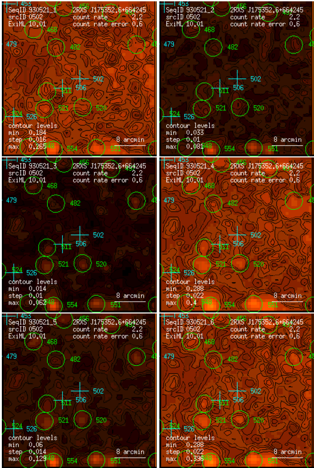
Figure 502: RASS 930521: detection 0502: band rate images, Gaussian filter: (1) PSPC channels 11 – 41, (2) 52 – 90, (3) 91 – 201, (4) 11 – 235, (5) 52 – 201, (6) 11 – 201. Broad band rates in counts/ks. Band rate contour levels in counts/ks/arcmin 2 .
